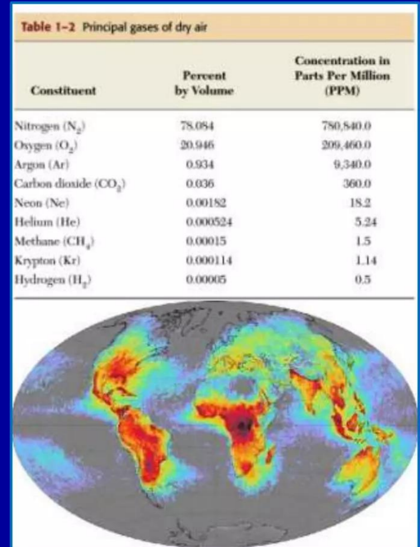
Map: lightning flash frequency
