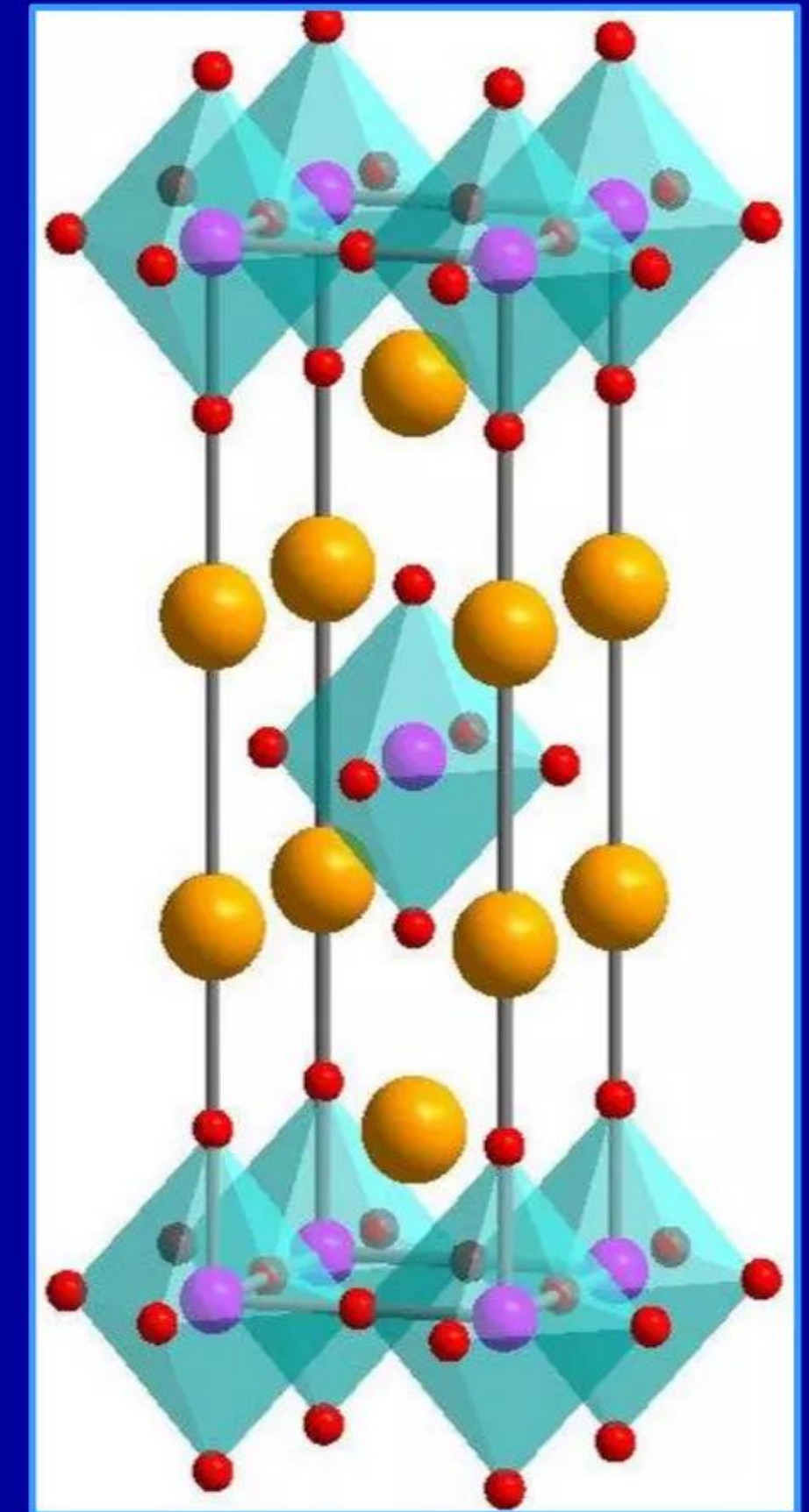
Credit: Y. Liu (Penn State Univ.) p-wave superconductor: \text{Sr}_2\text{RuO}_4
