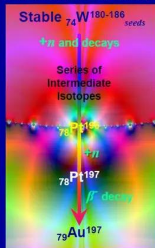
Example 1 Production of Gold: one possible path
