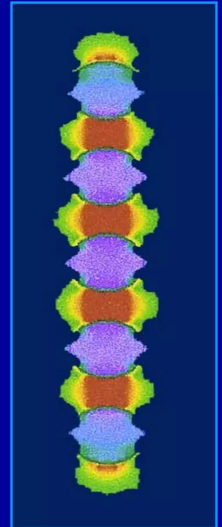
Surface Plasmon Fields Around Nanoparticles
