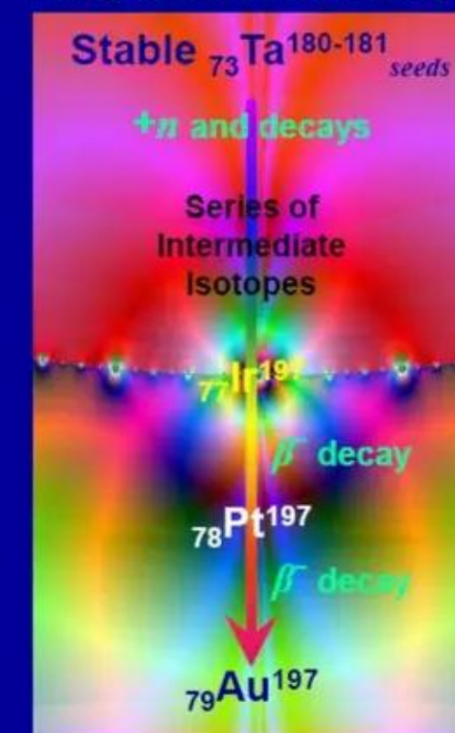
Example 2 Making Gold: another possible path
