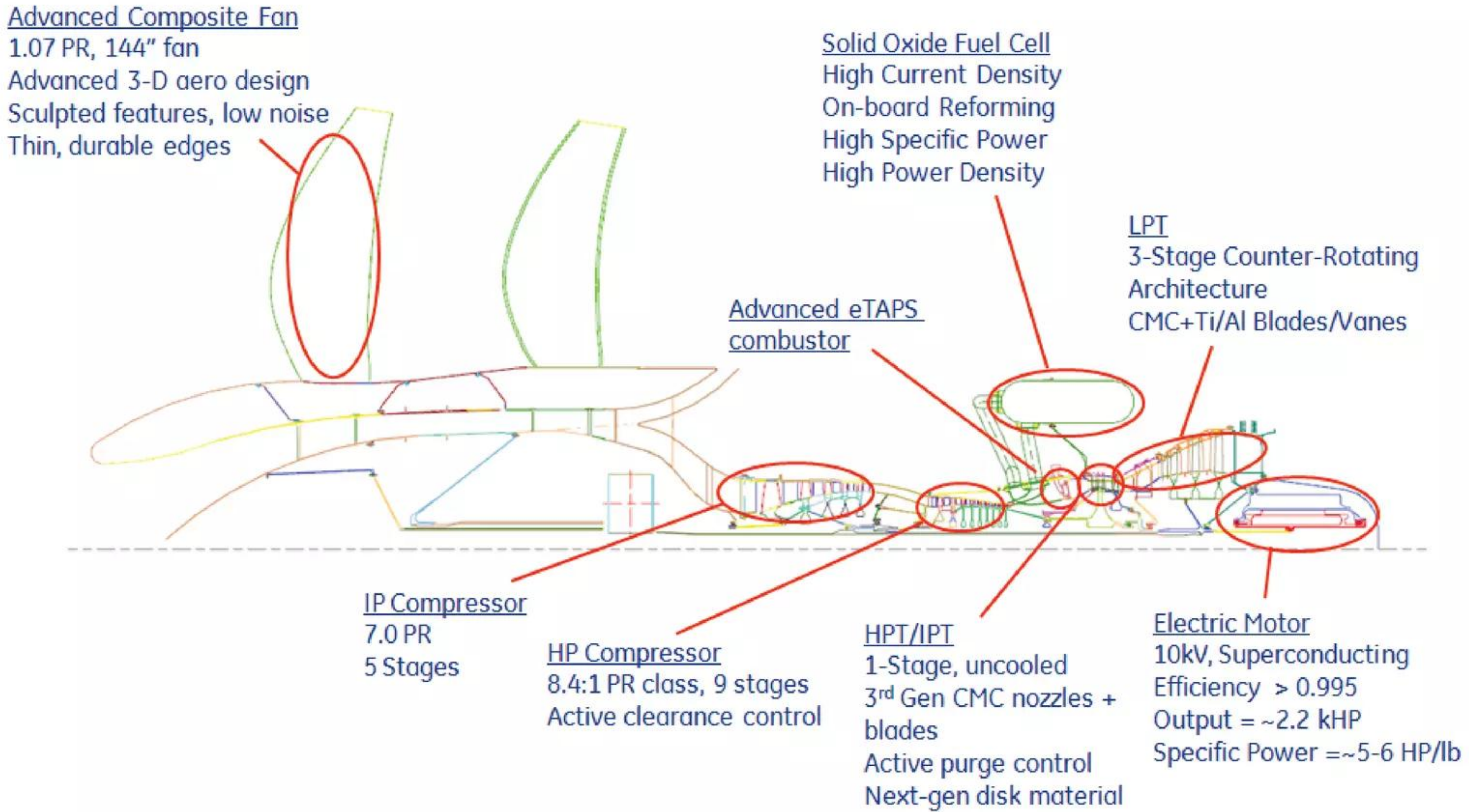
Figure 3 - LNG+2045GT+SOFC+UDF Concept Layout
