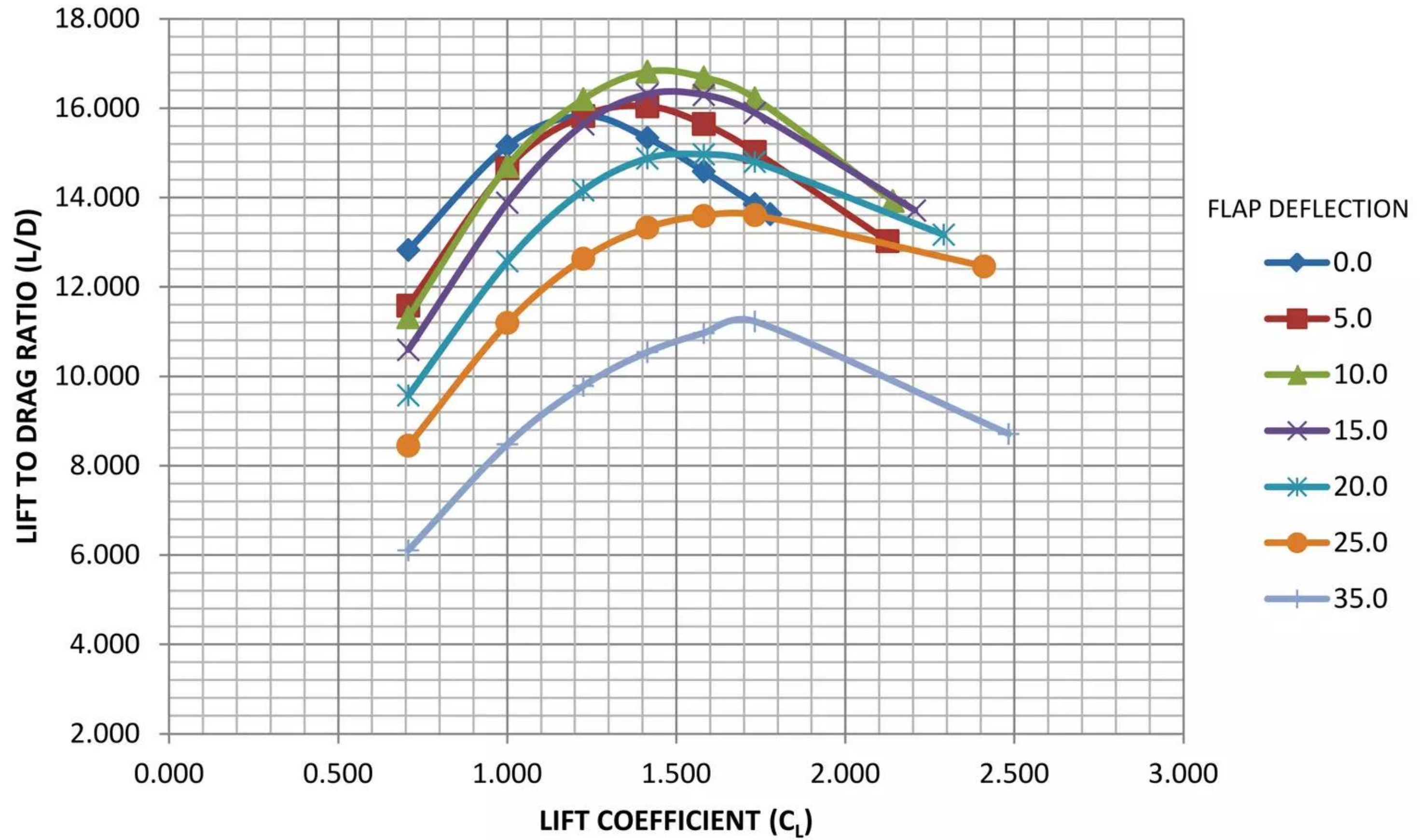
Figure 5.11 – 765-095-TS1 - Low Speed Lift / Drag; Free Air
