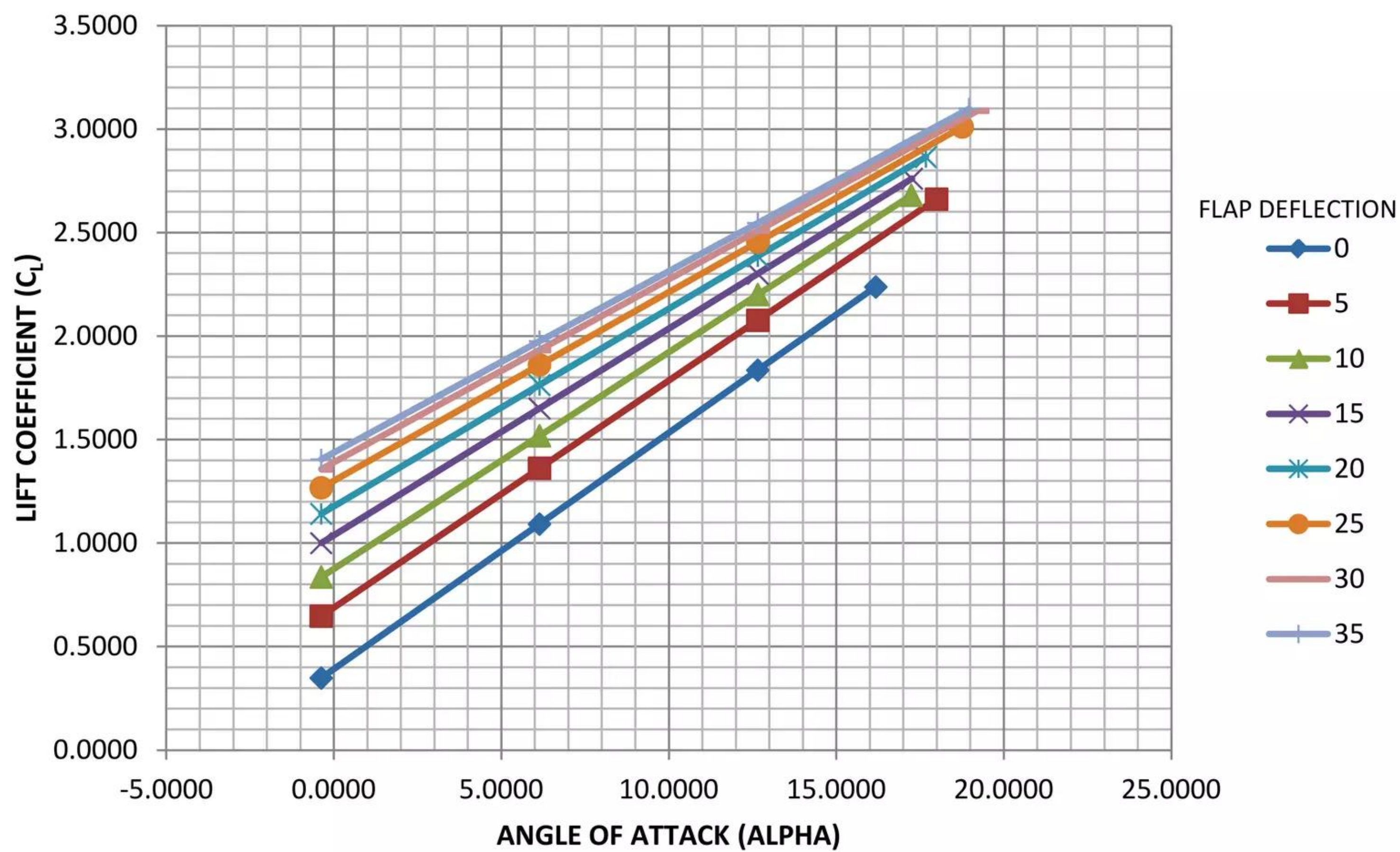
Figure 5.3 – 765-094-TS1 - Low Speed Lift Curve; Free Air
