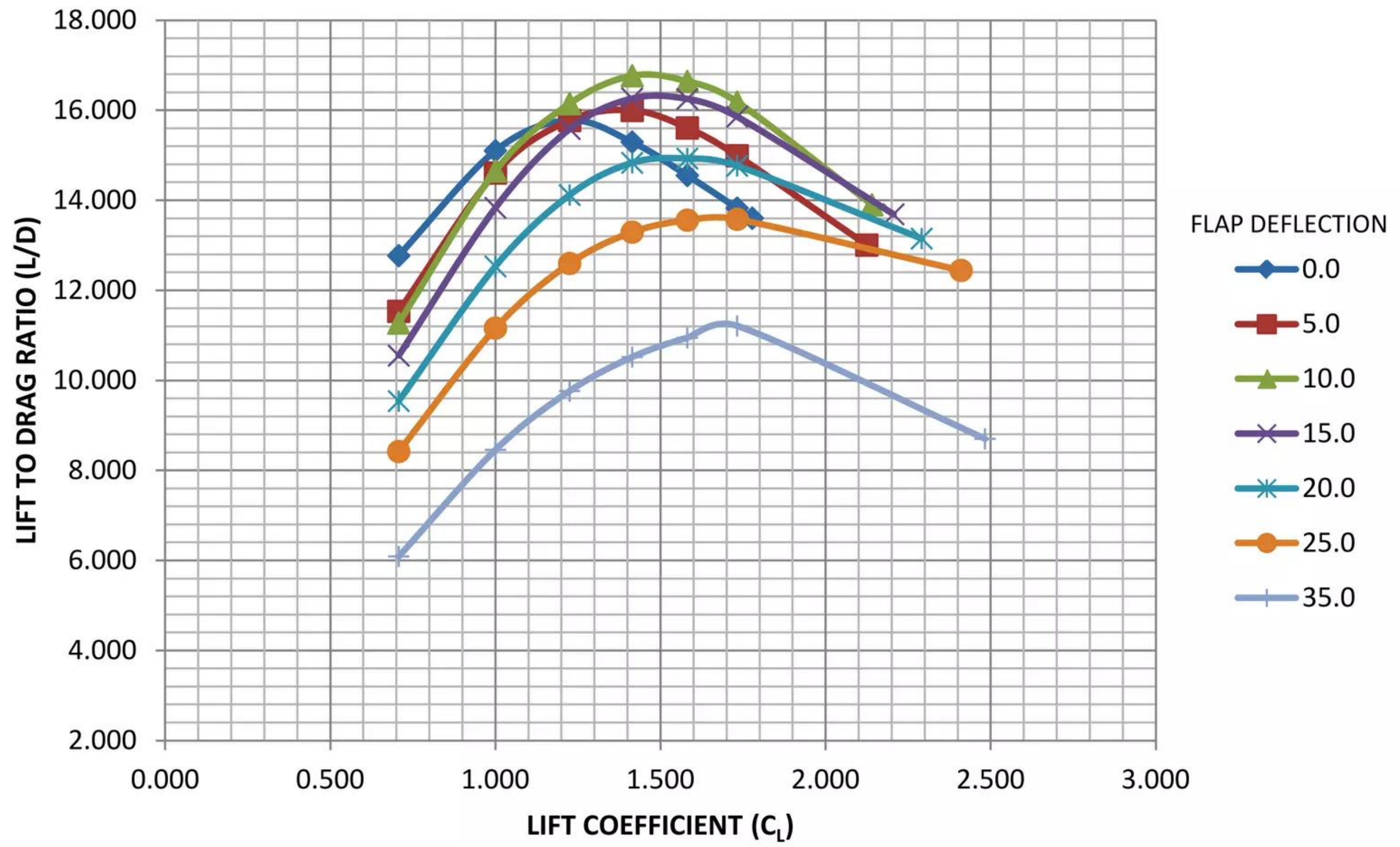
Figure 5.18 – 765-095-TS2 - Low Speed Lift / Drag; Free Air
