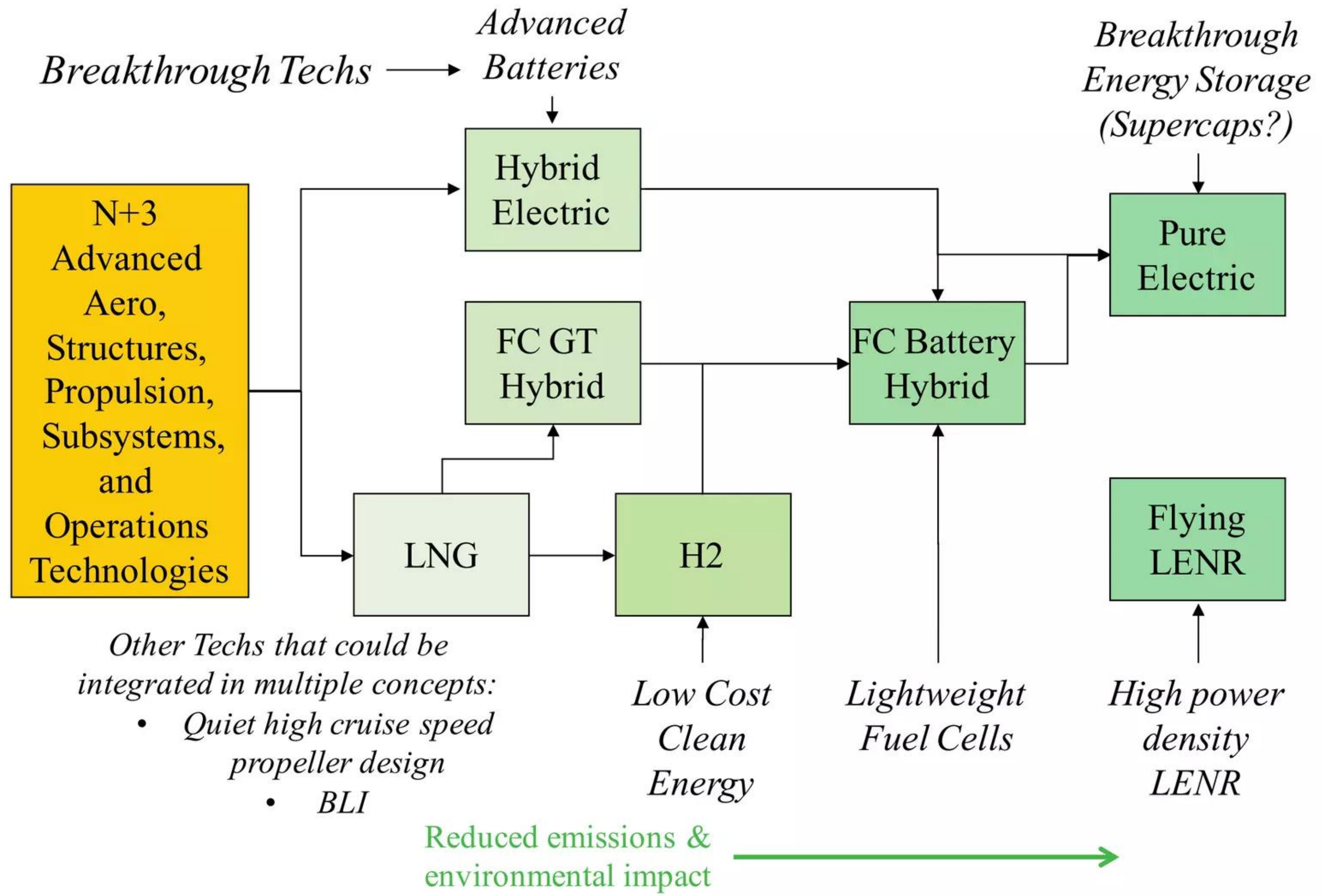
Figure 2.11 – Relationship of N+4 Workshop Technologies
