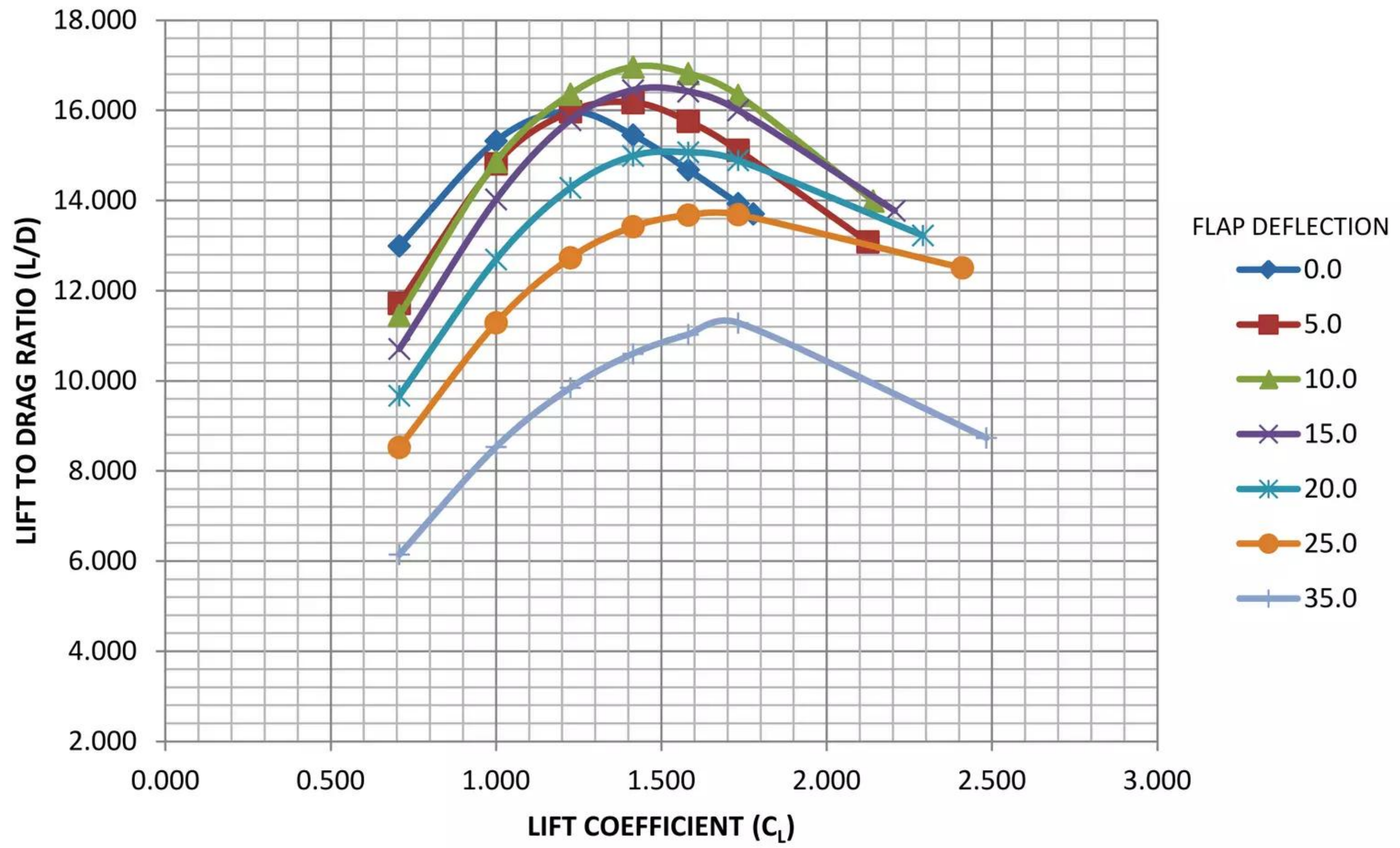
Figure 5.24 – 765-095-TS3 - Low Speed Lift / Drag; Free Air
