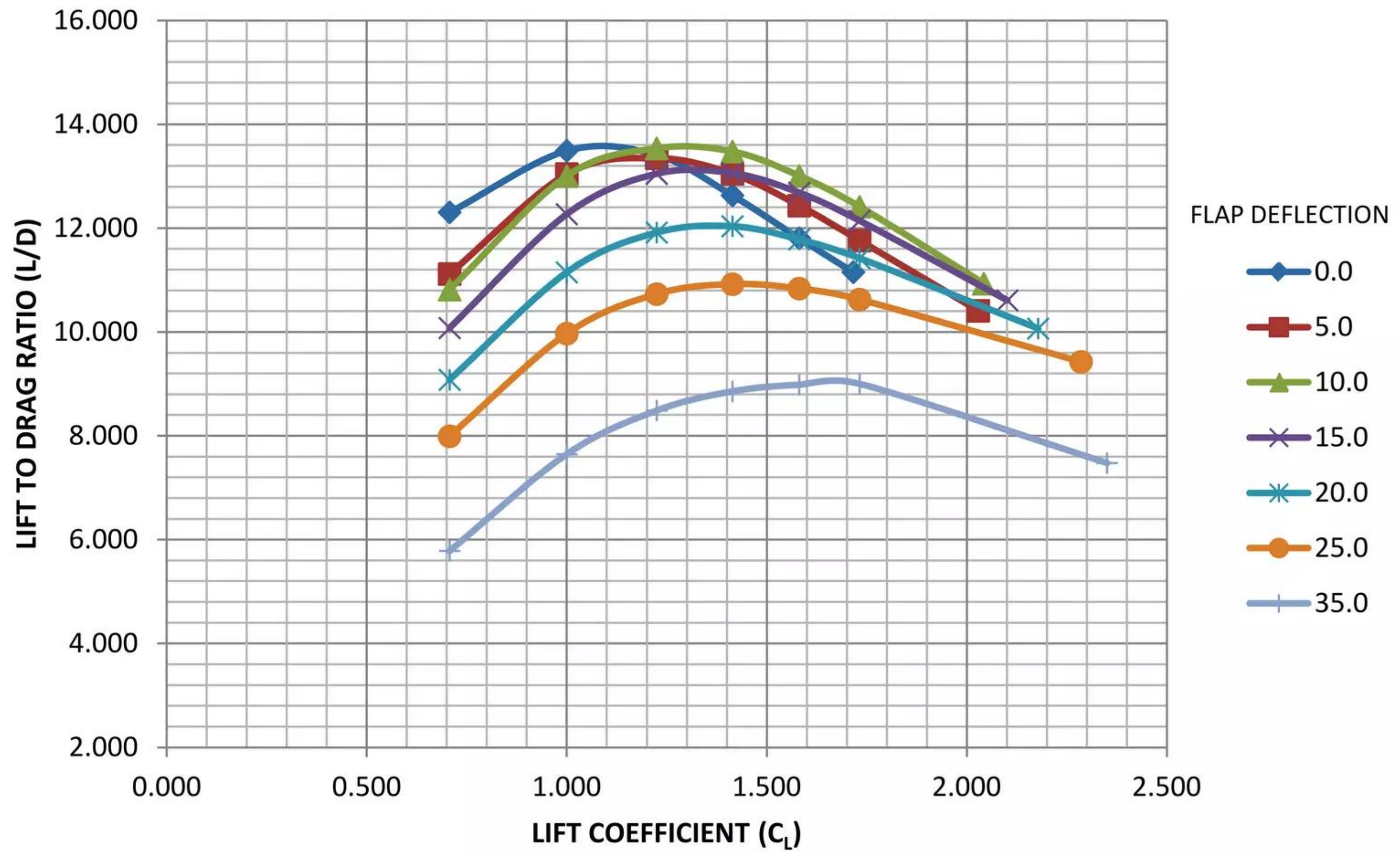
Figure 5.5 – 765-094-TS1 - Low Speed Lift / Drag; Free Air
