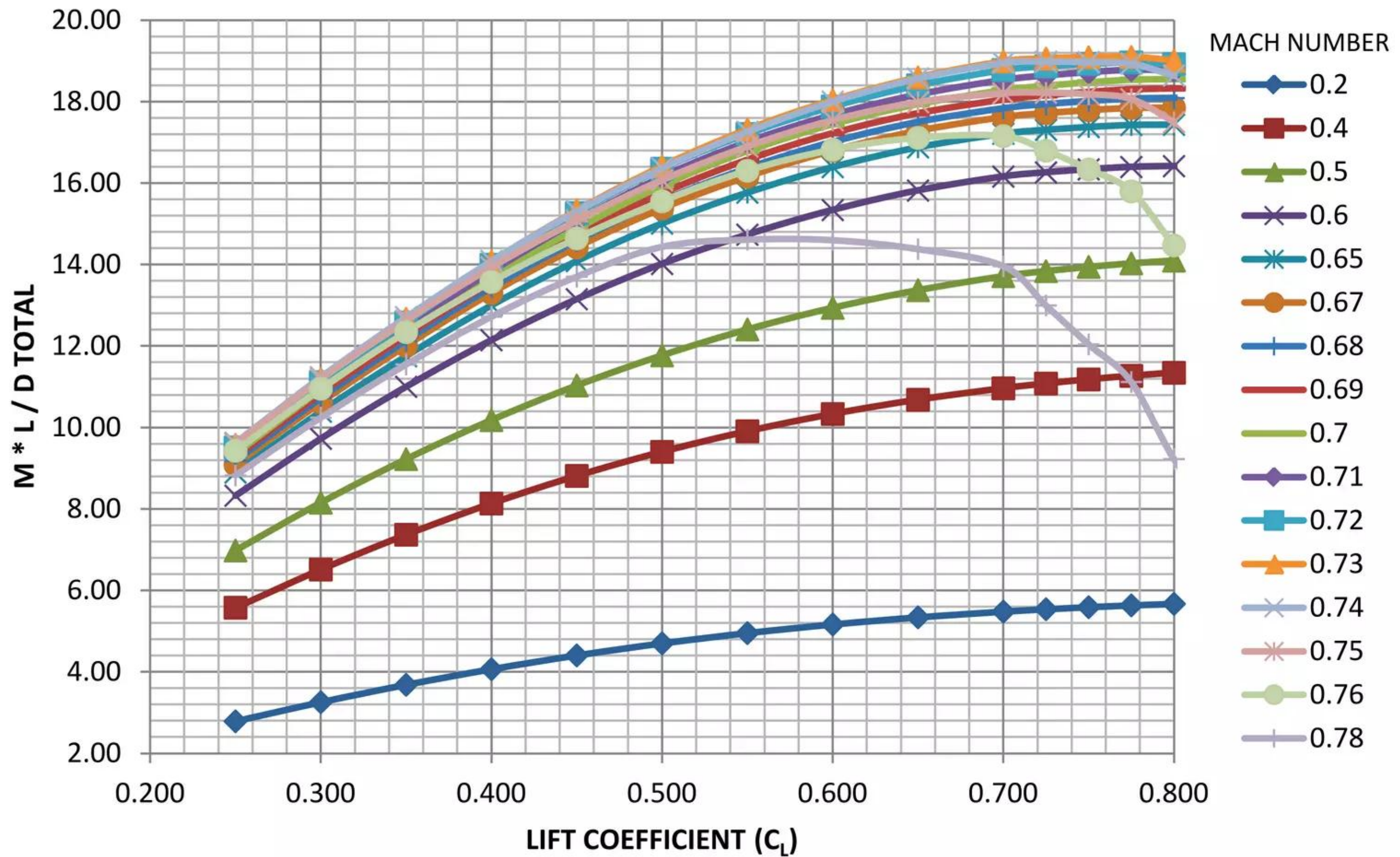
Figure 5.8 – 765-095-TS1 - M \cdot L / D \text{ Total}
