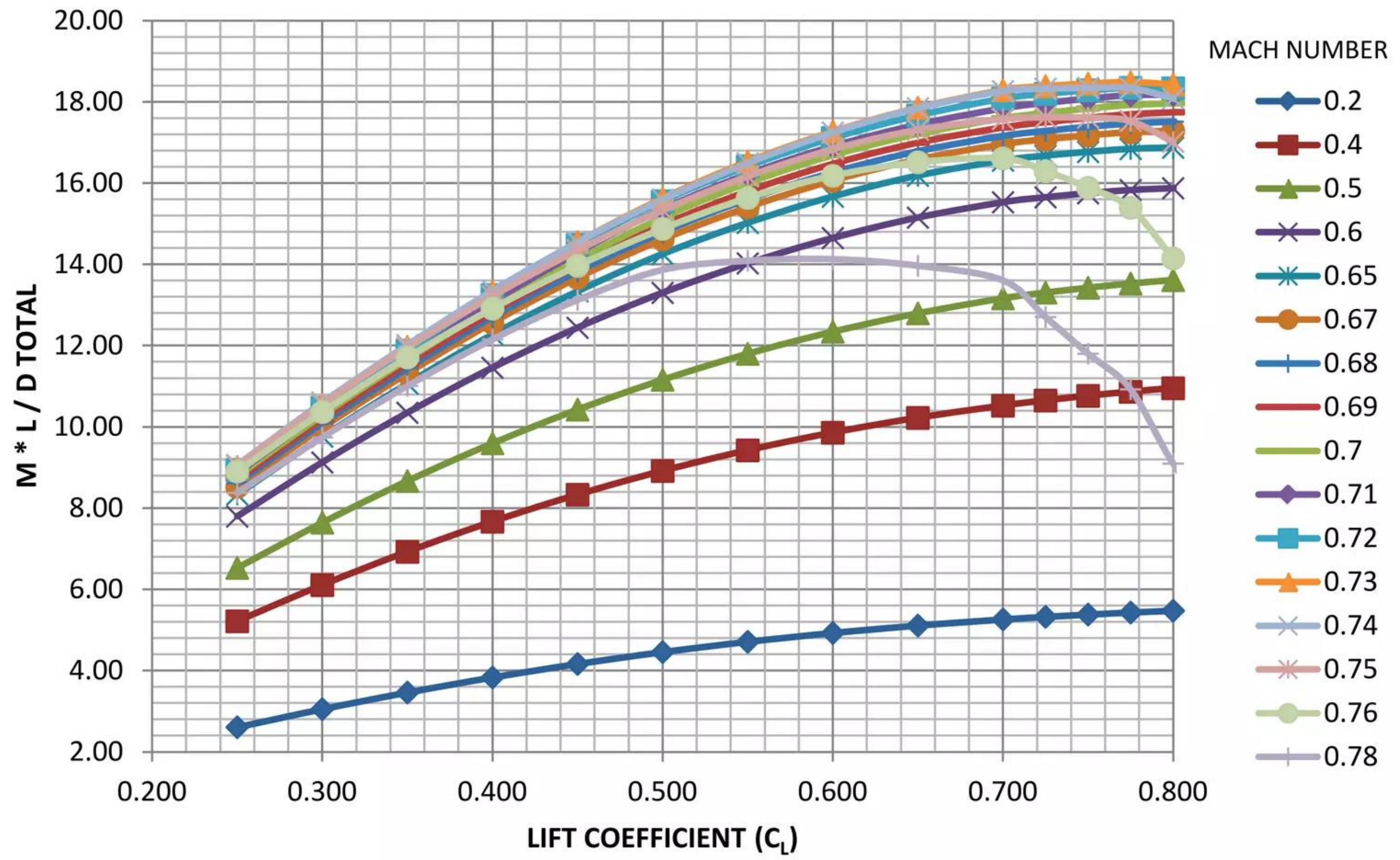
Figure 5.21 – 765-095-TS3 - M * L / D Total
