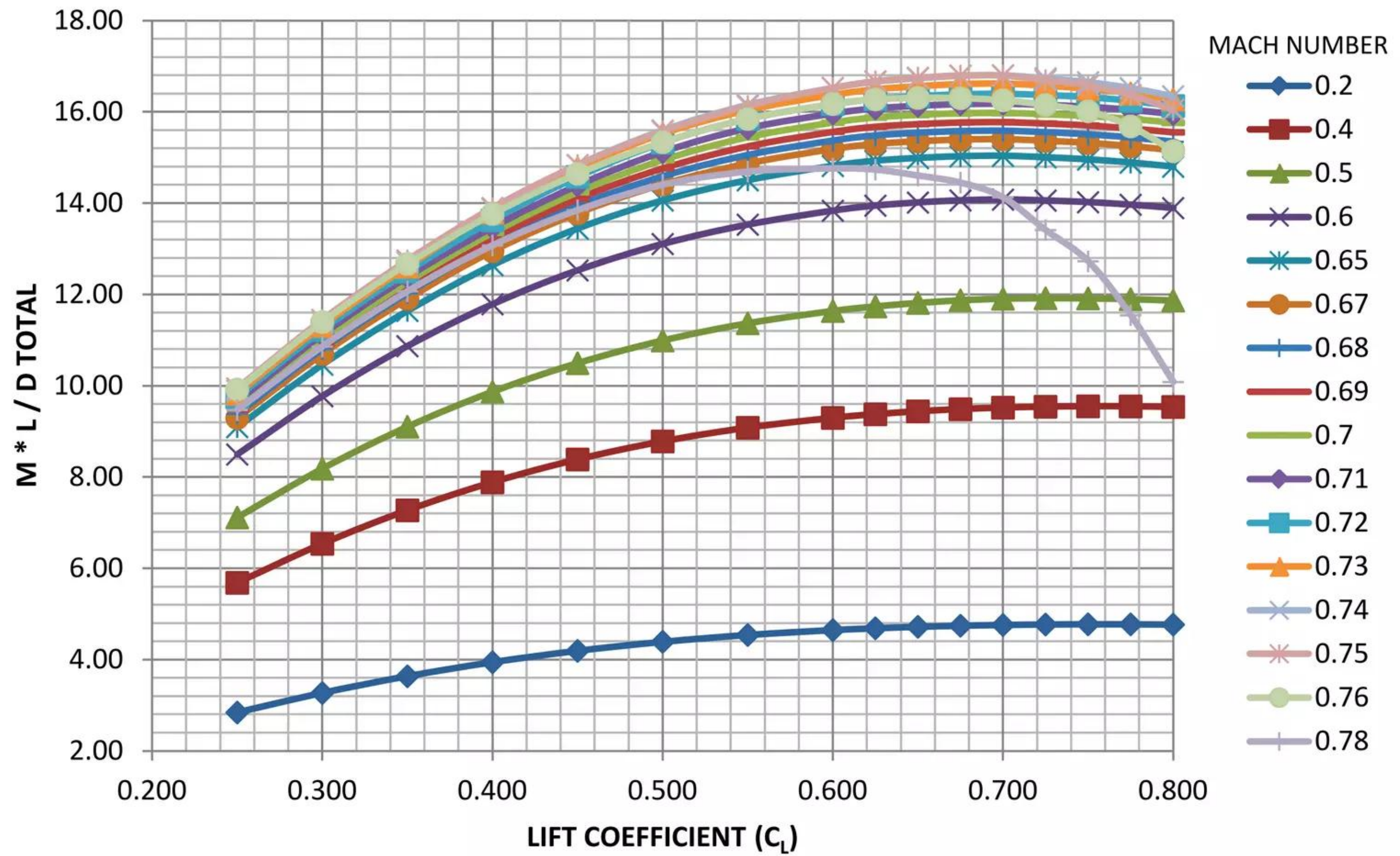
Figure 5.2 – 765-094-TS1 - M * L / D Total
