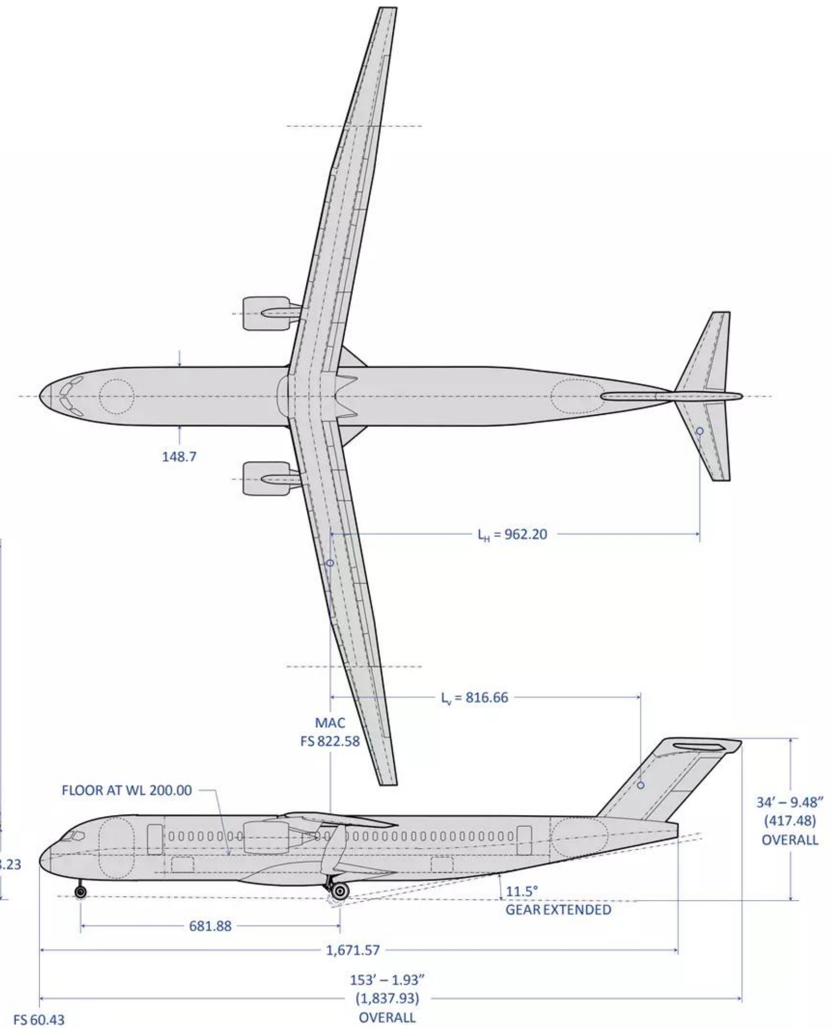
Figure 5.13 – 765-095-TS2 – Truss Braced Wing With LNG gFan++
