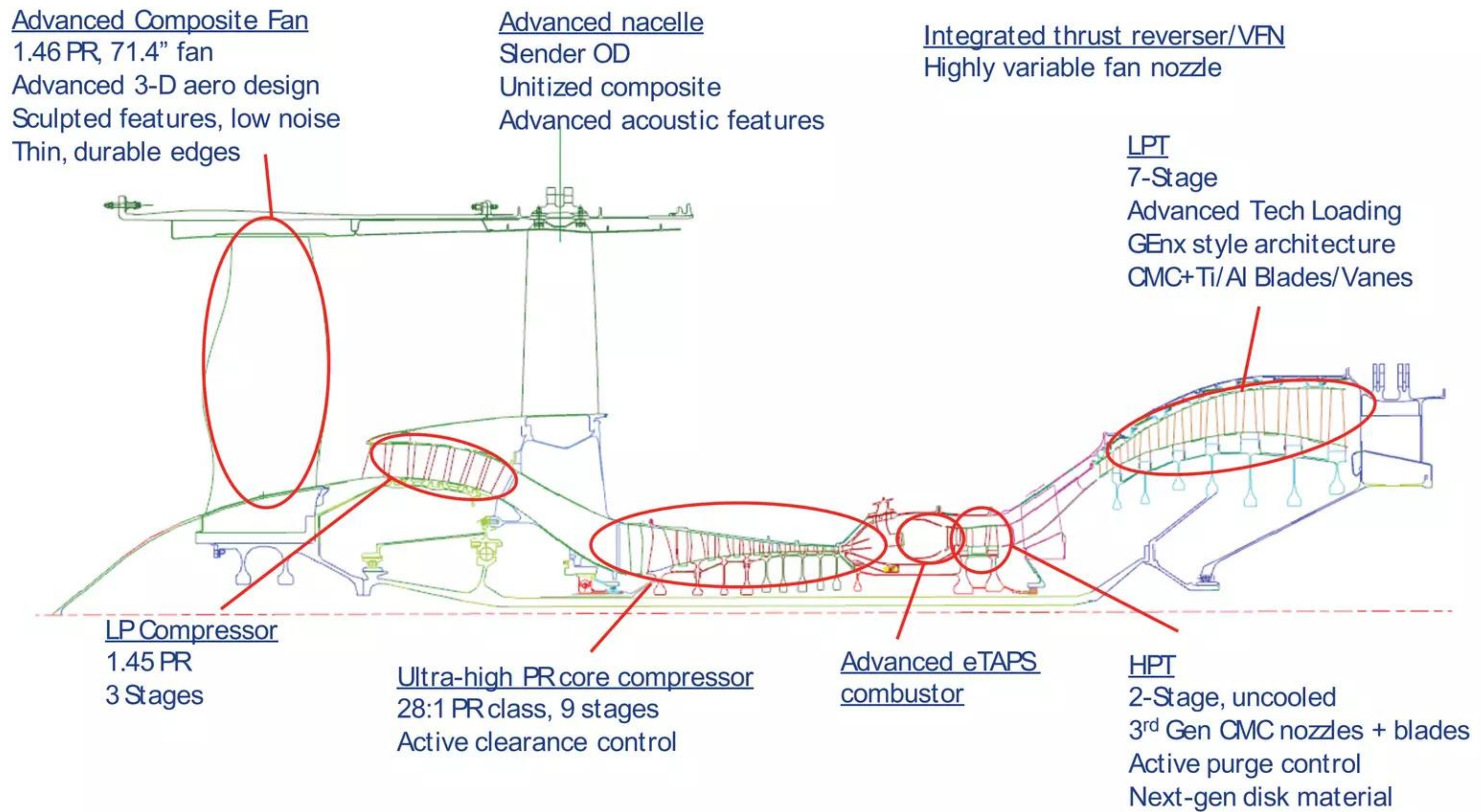
Figure 2- gFan++ (JP+2045GT+DF) Concept Layout
