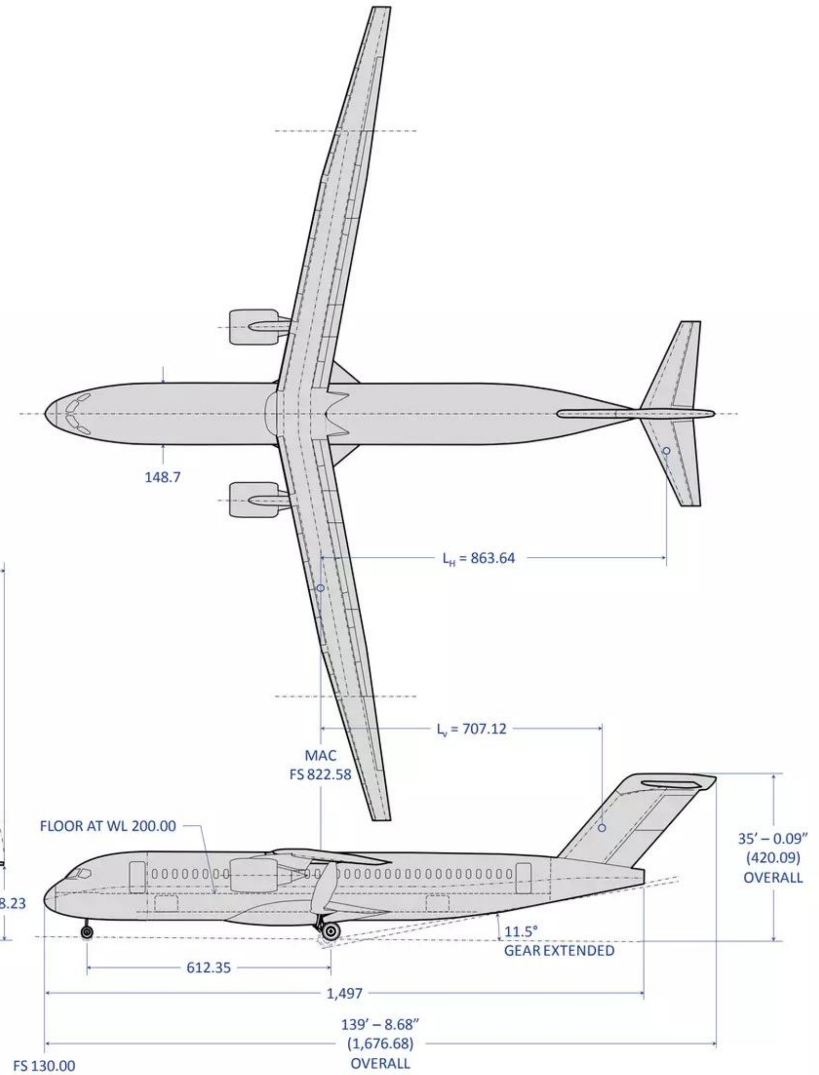
Figure 5.6 – 765-095-TS1 – Truss Braced Wing with gFan++
