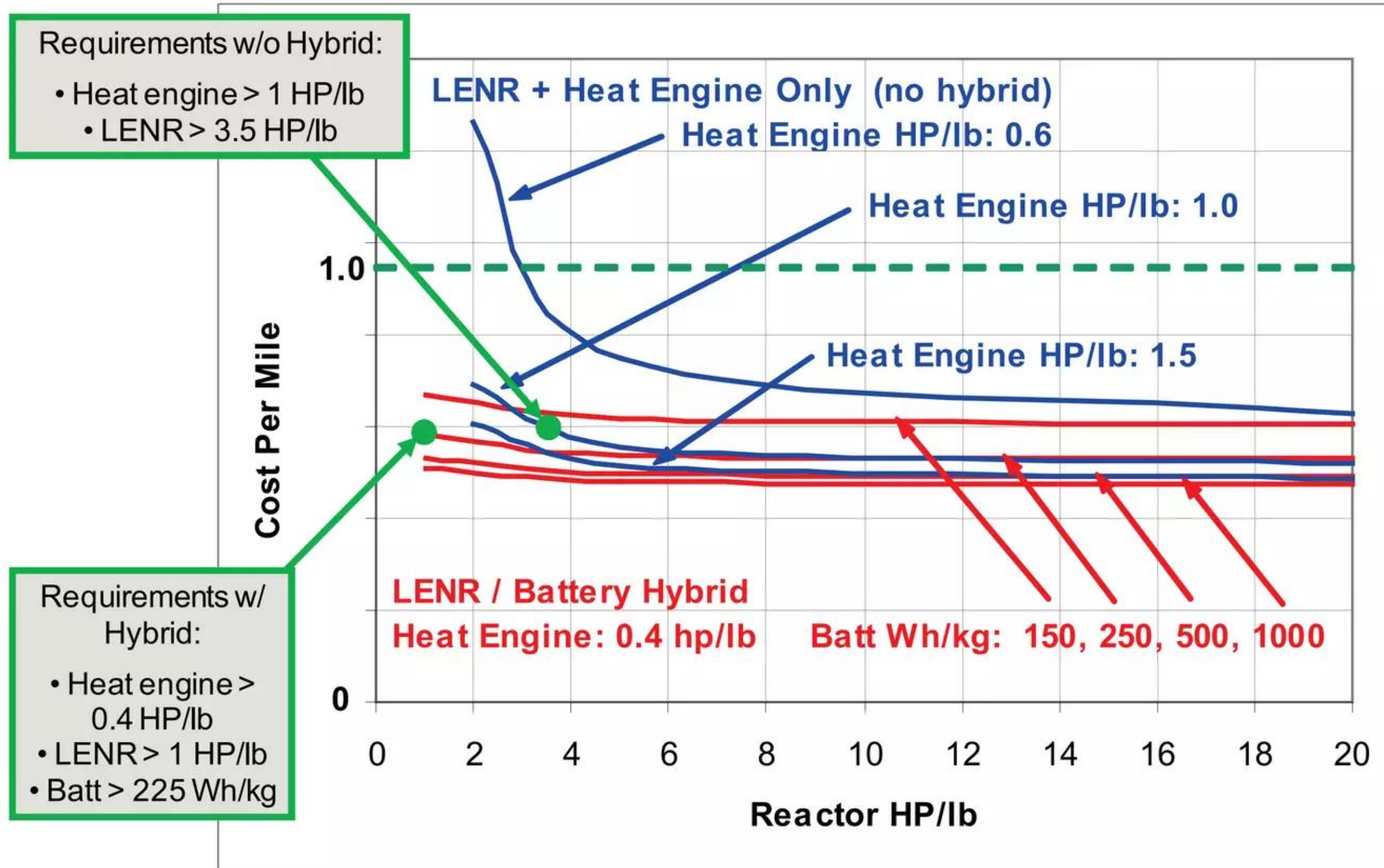
Figure 3.3 – Hybrid LENR + Battery Performance Parameters
