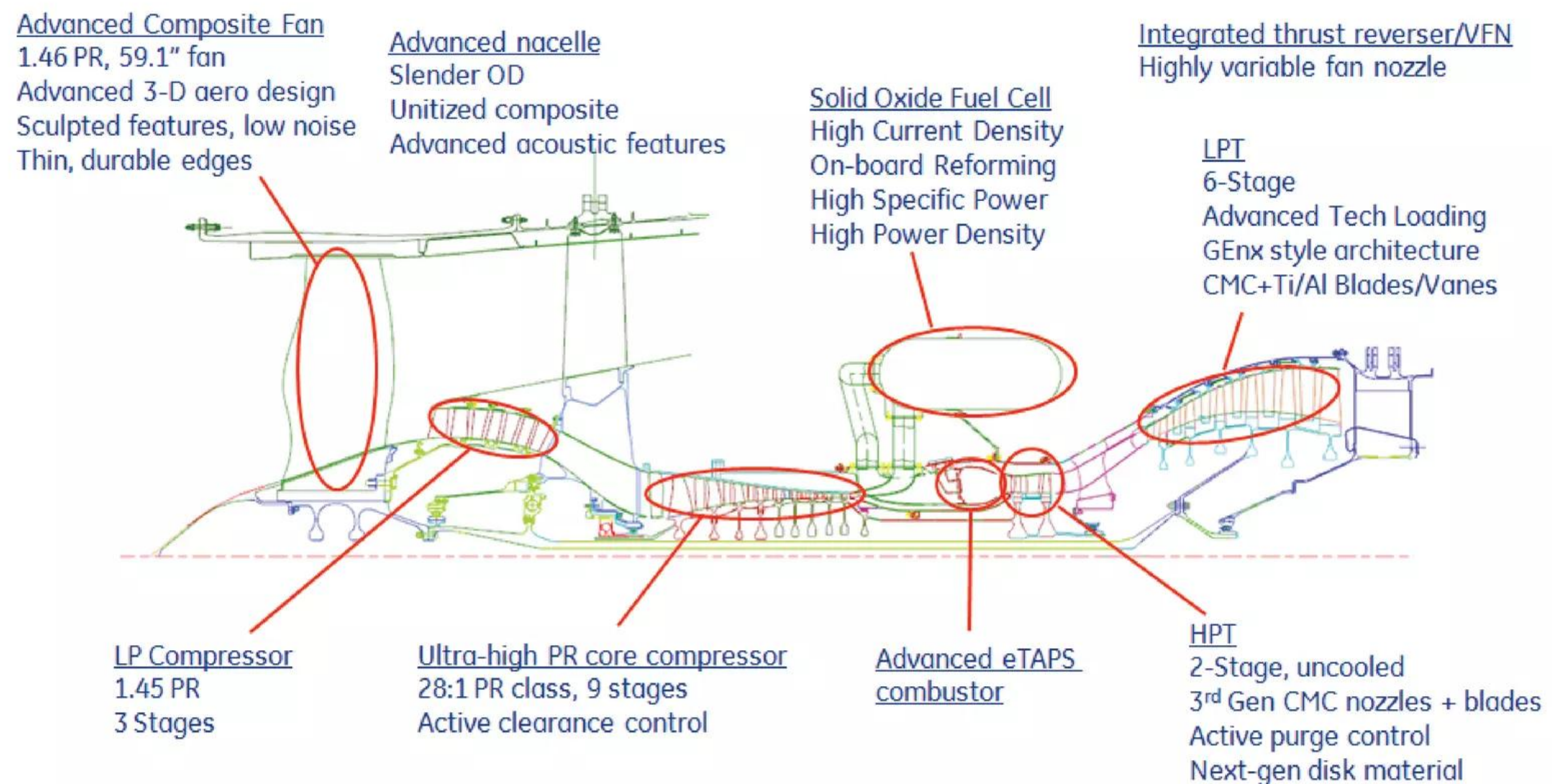
Figure 4 - LNG+2045GT+SOFC+DF+BLI (Wing Fans)
