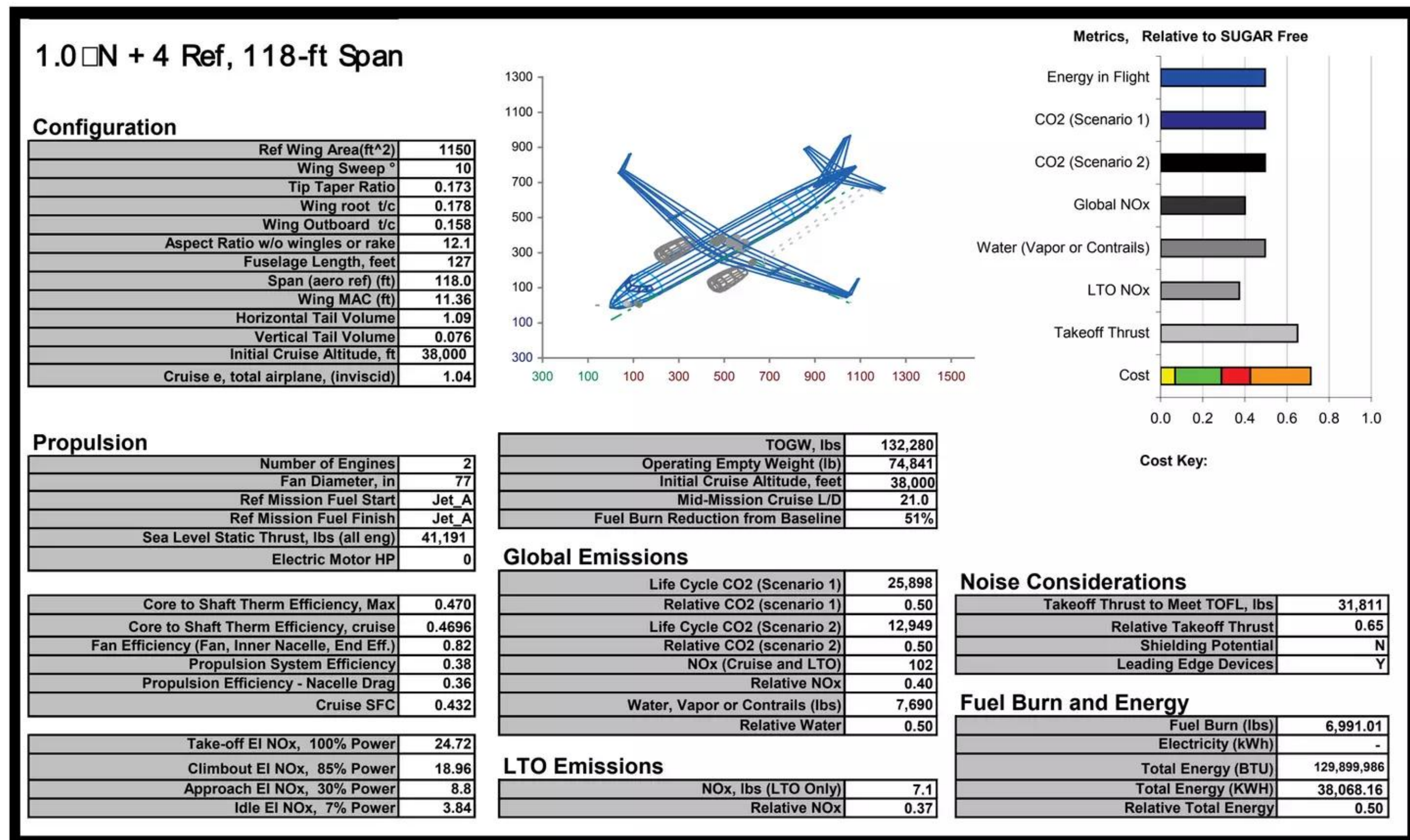
Figure 2.7 – N+4 Workshop Concept Overview Template
