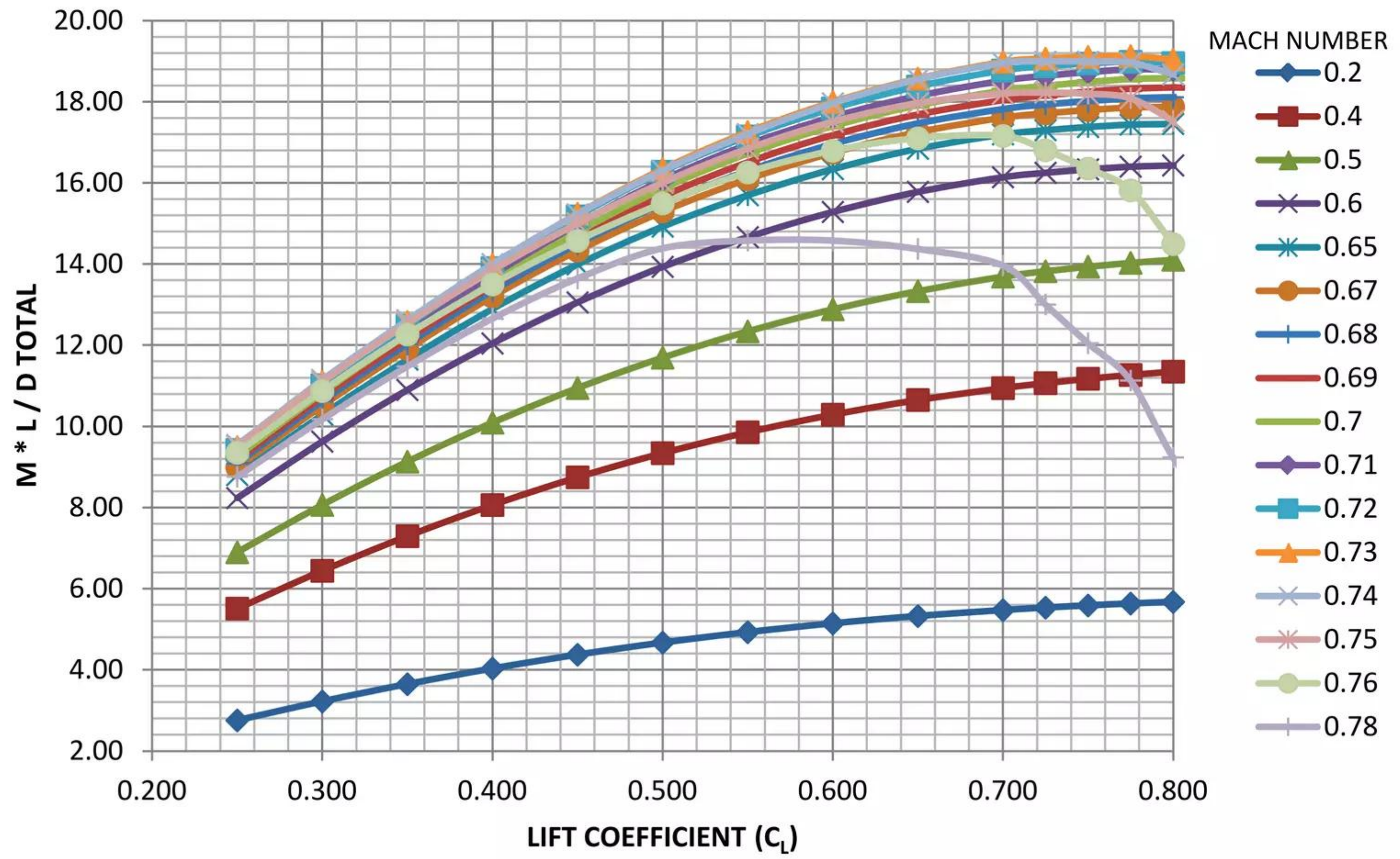
Figure 5.15 – 765-095-TS2 - M * L / D_{Total}
