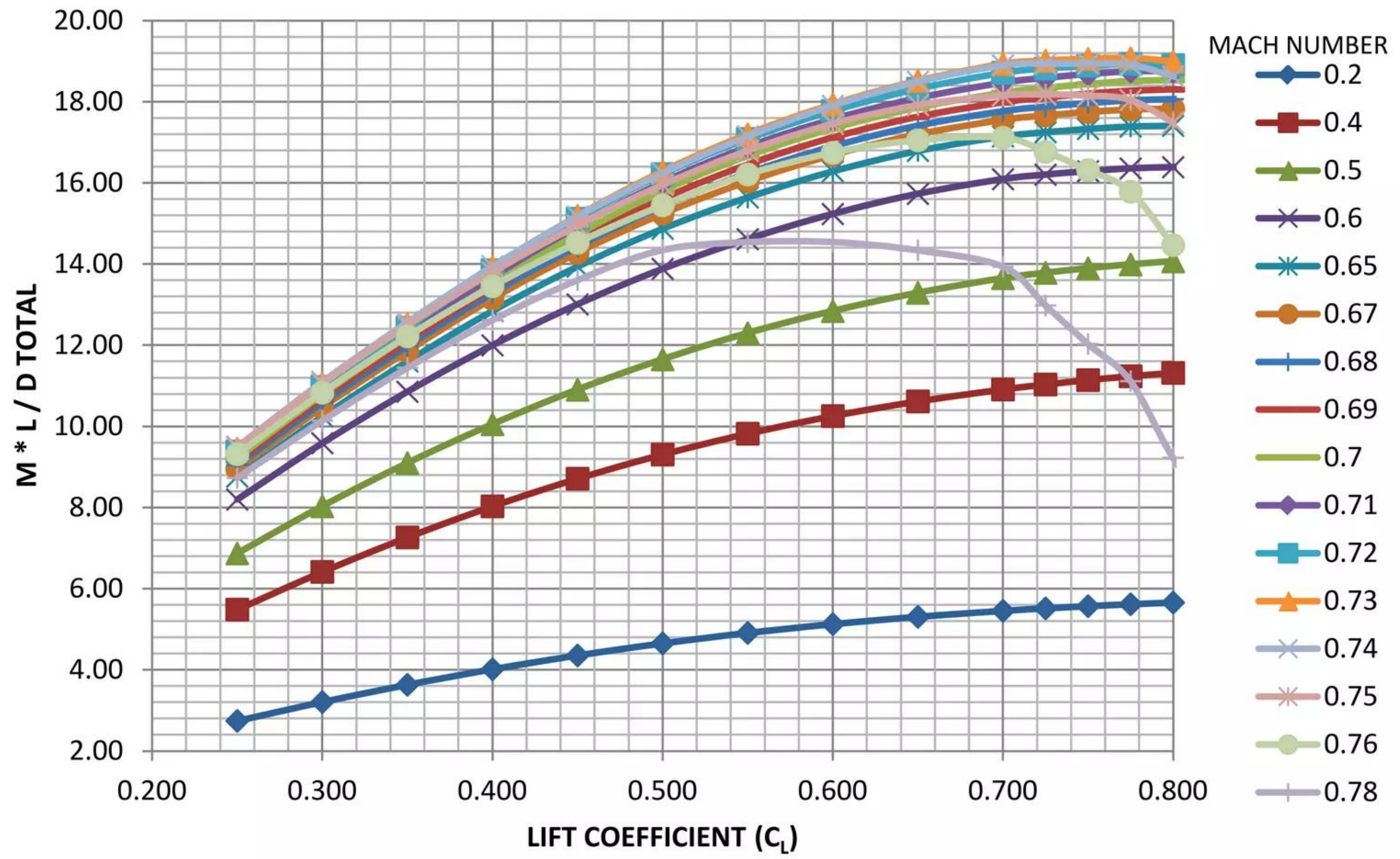
Figure 5.28 – 765-095-TS4 - M * L / D Total
