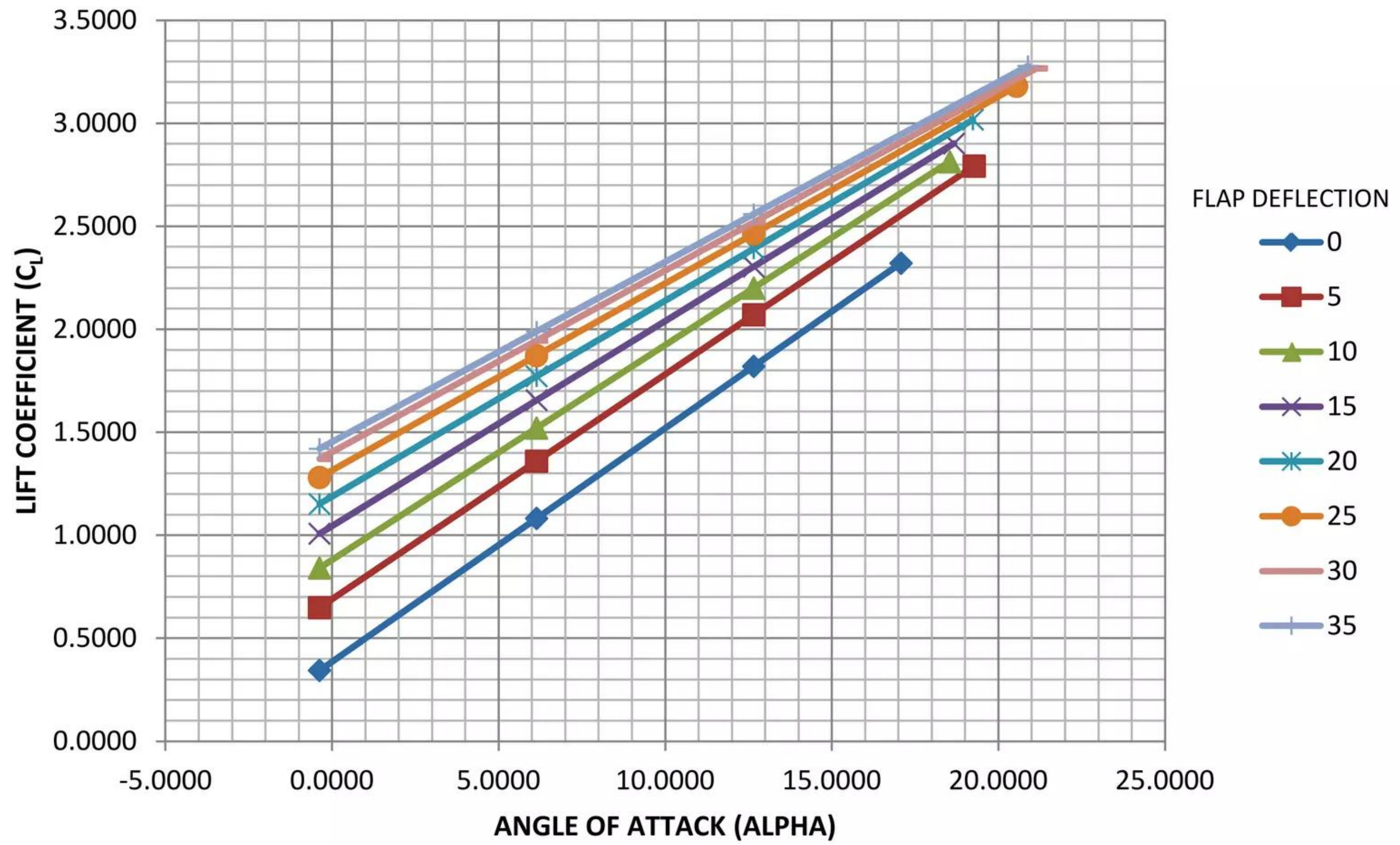
Figure 5.9 – 765-095-TS1 - Low Speed Lift Curve; Free Air
