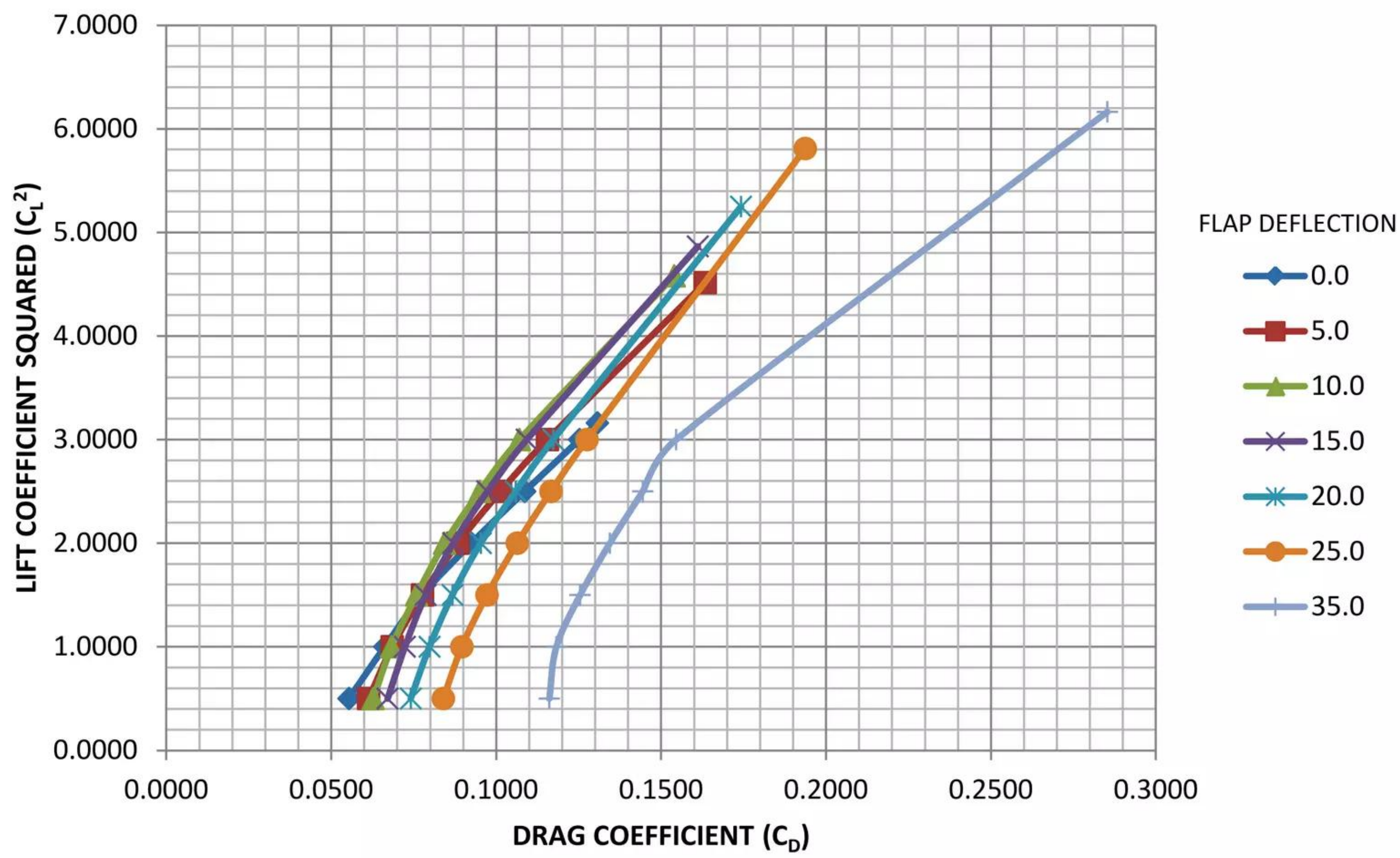
Figure 5.16 – 765-095-TS2 - Low Speed Lift Curve; Free Air
