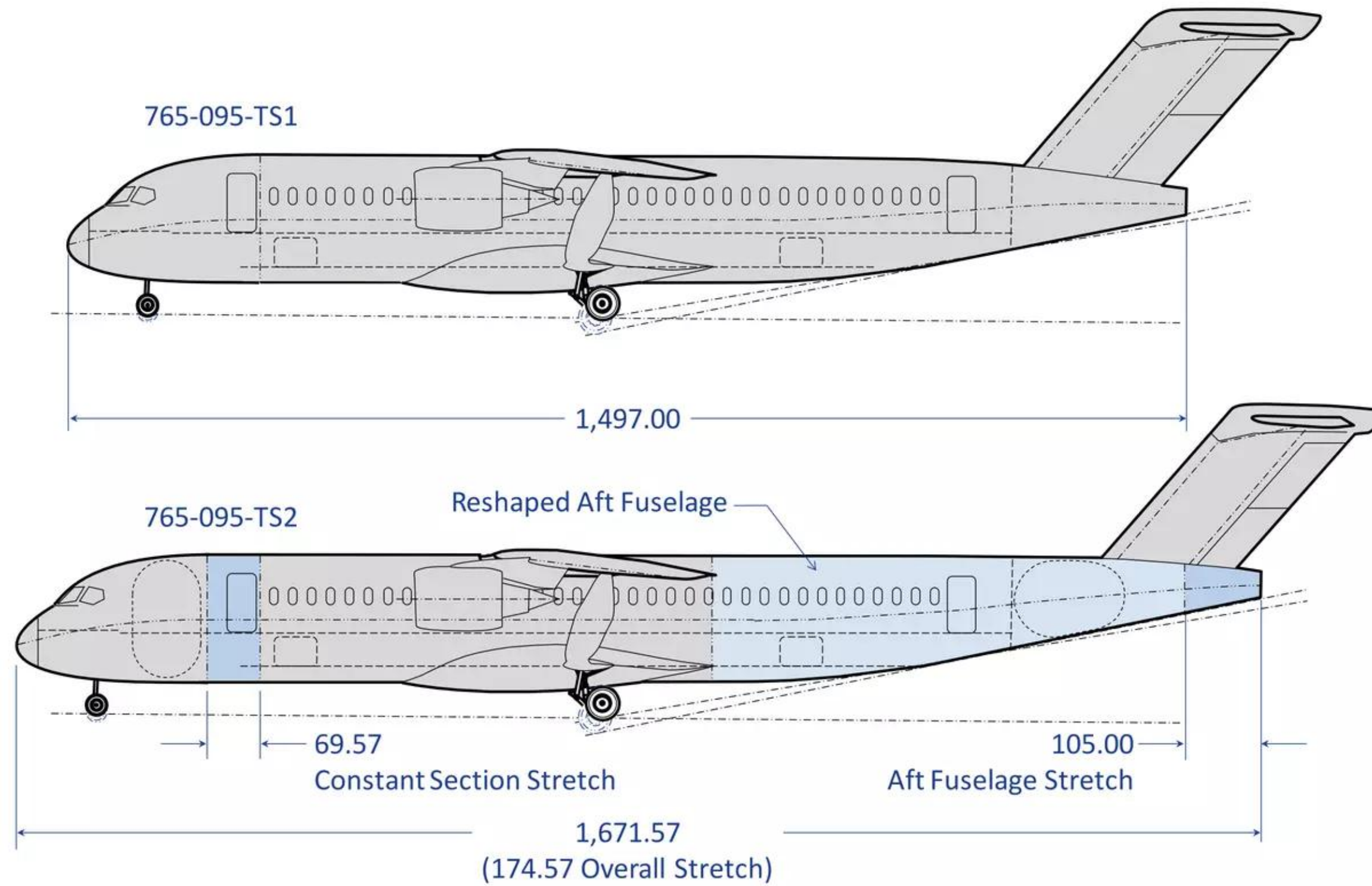
Figure 5.12 – Fuselage Stretched to Accommodate LNG Tankage
