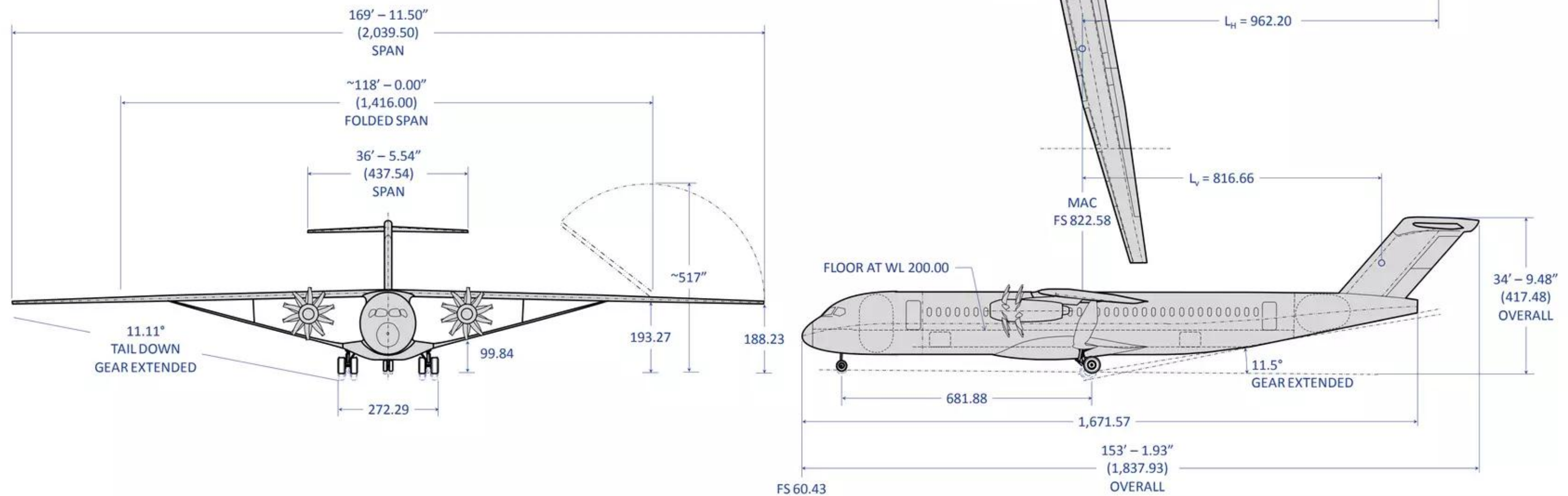
Figure 5.19 – 765-095-TS3 - Truss Braced Wing With LNG UDF
