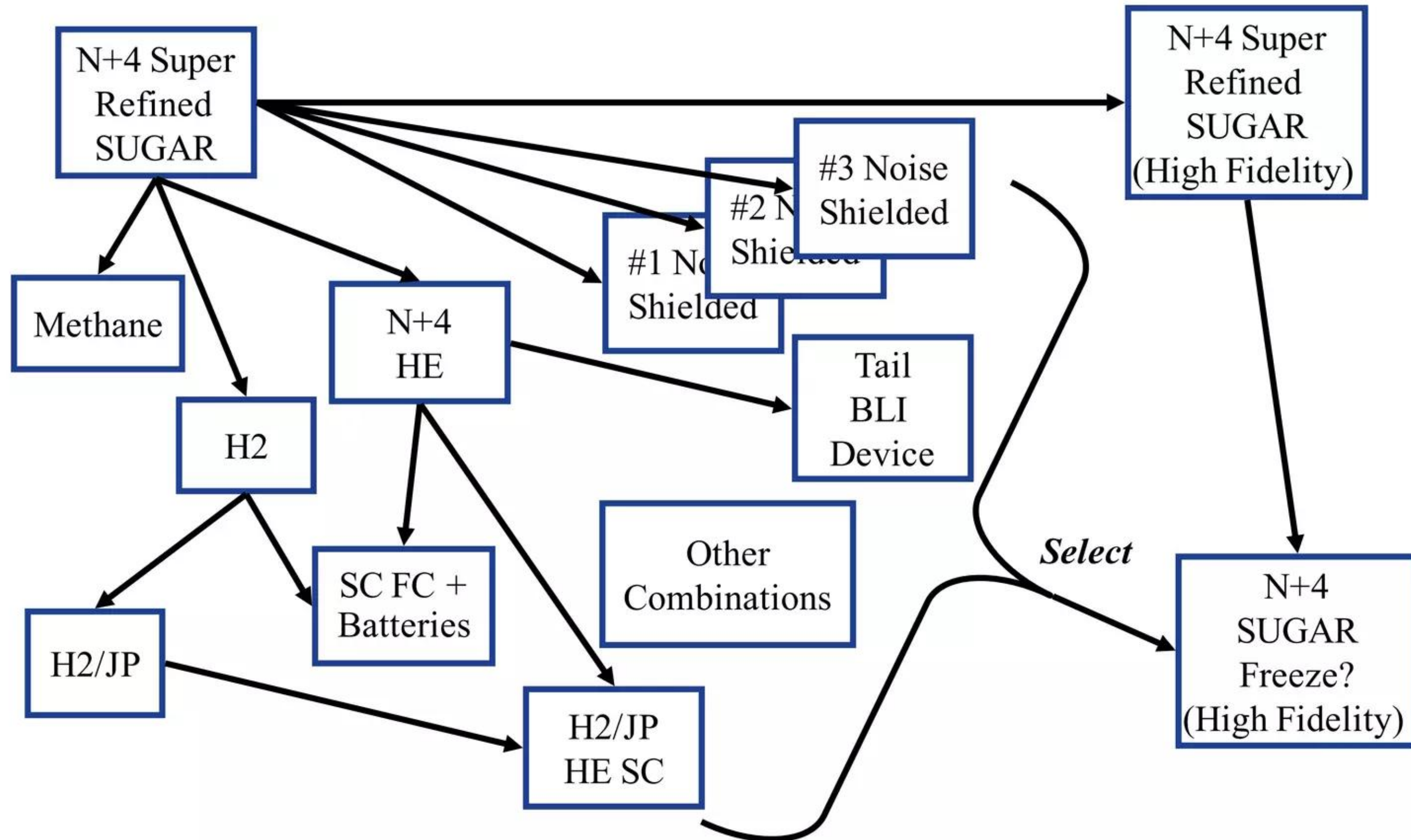
Figure 2.2 – N+4 Configuration Analysis Flow
