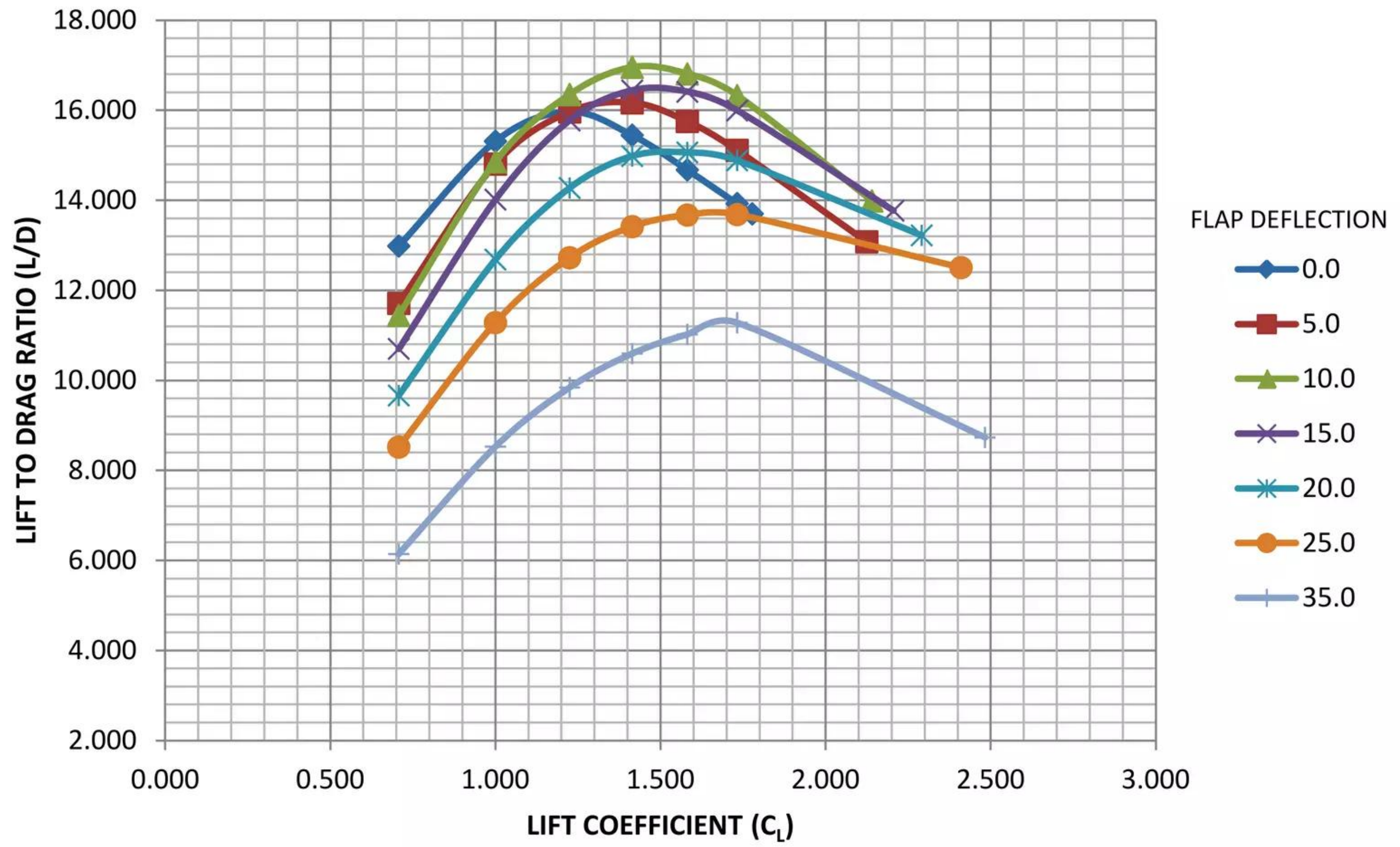
Figure 5.31 – 765-095-TS4 - Low Speed Lift / Drag; Free Air
