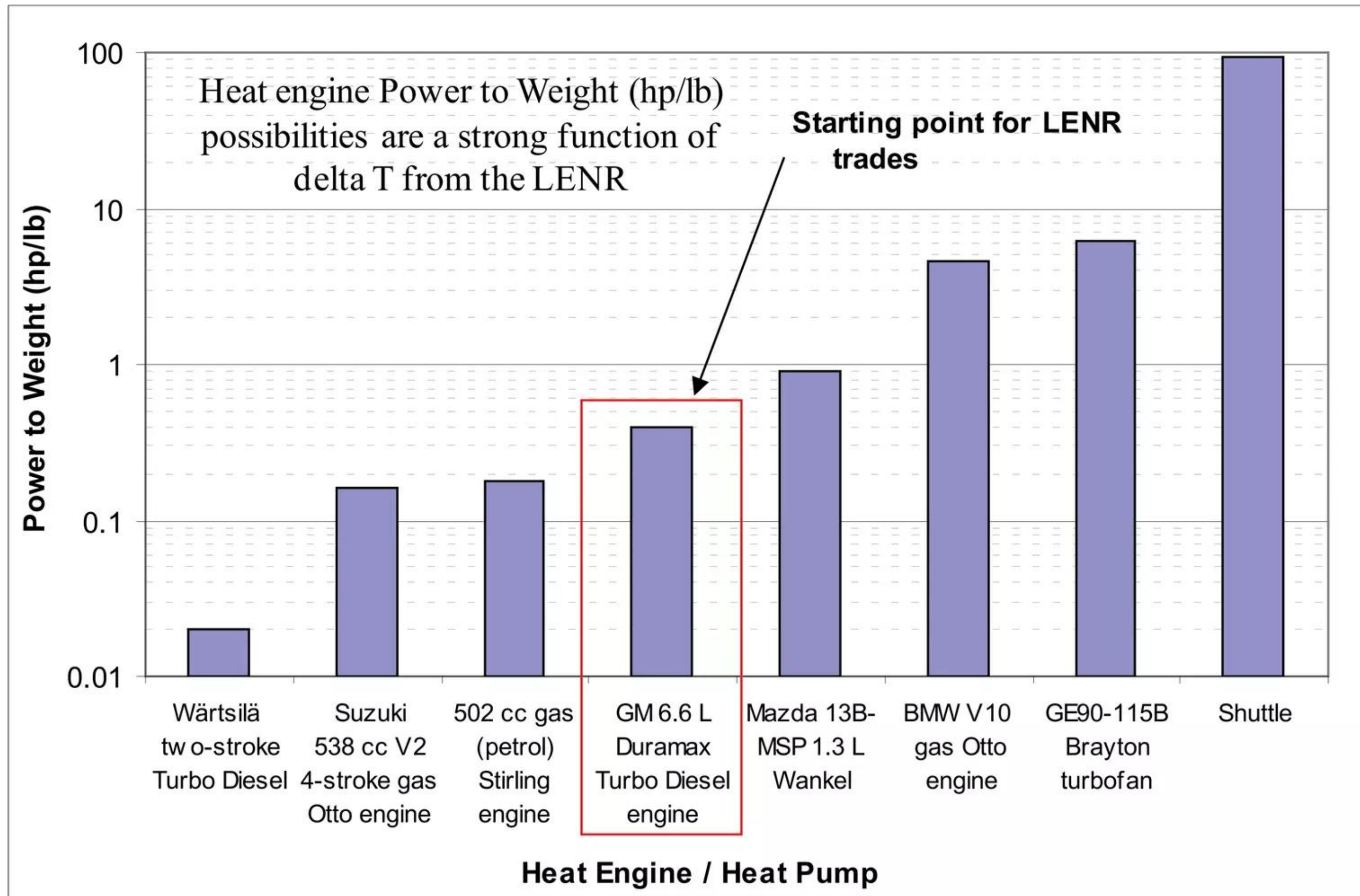
Figure 3.1 – Potential Heat Engines for LENR Systems
