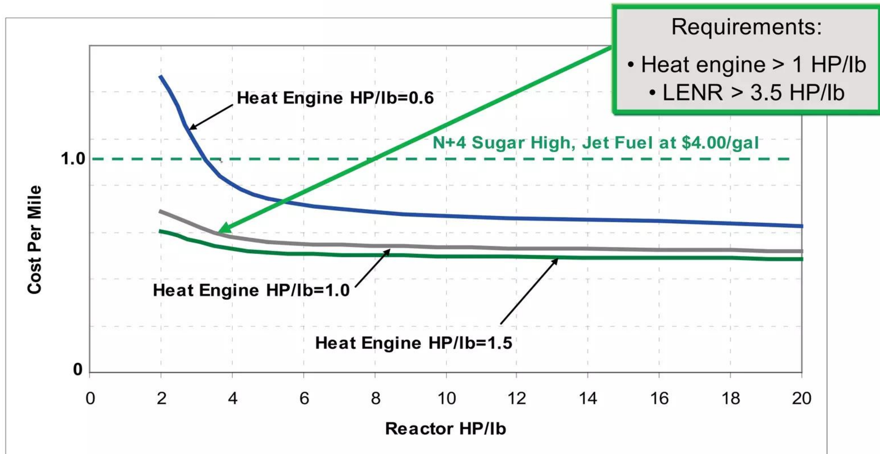
Figure 3.1 – Potential Heat Engines for LENR Systems
