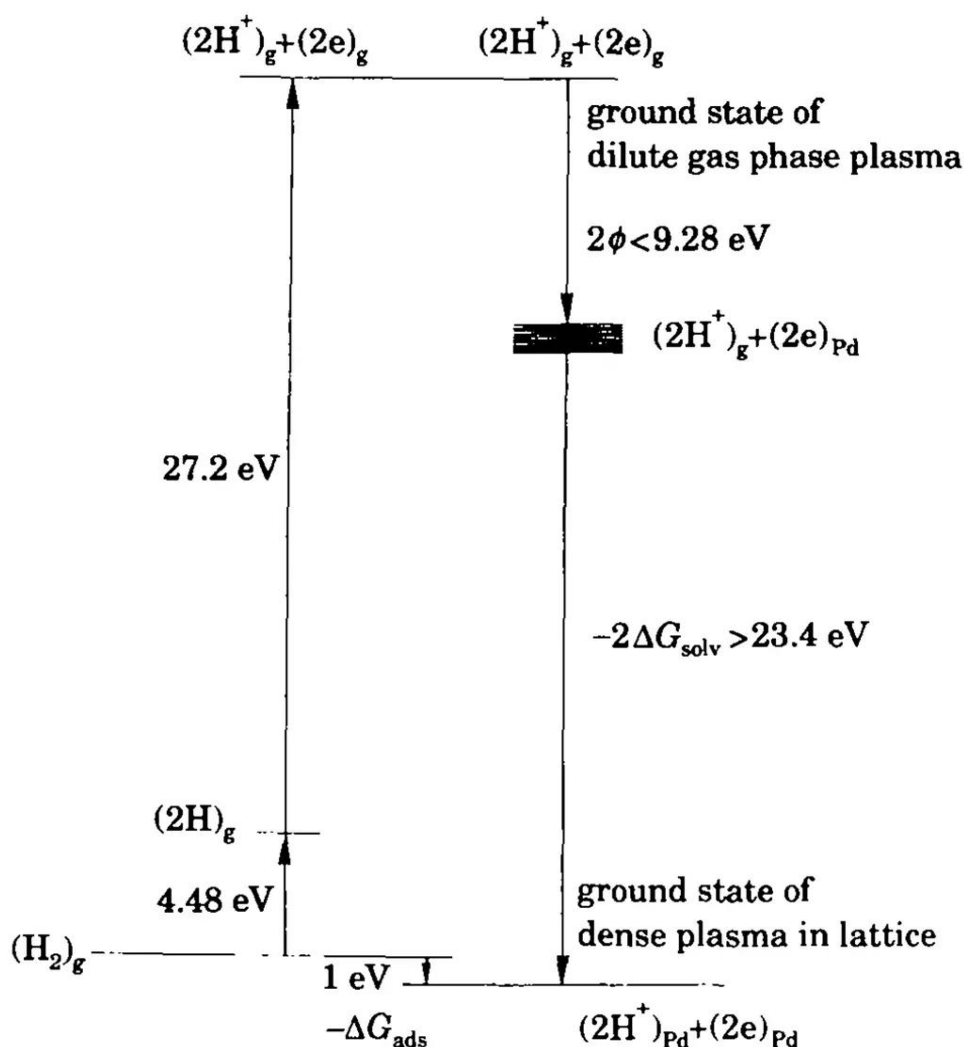
Fig. 1. – Yet another possible Born-Haber cycle for the \text{H}_2 absorption in metallic Pd.
