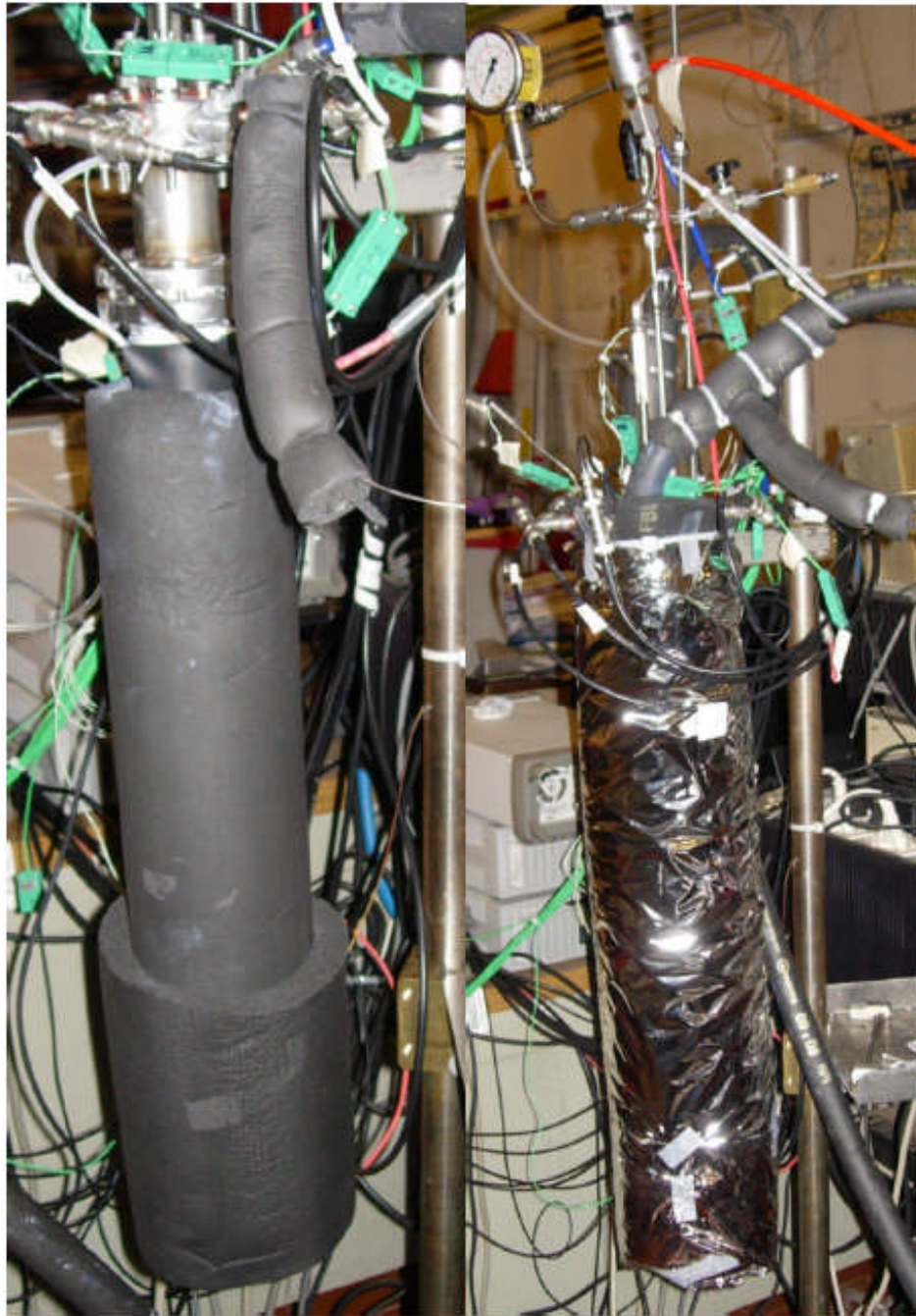
Figure 22. Real reactor: steps 6-7 of assembly, final thermal insulation.
