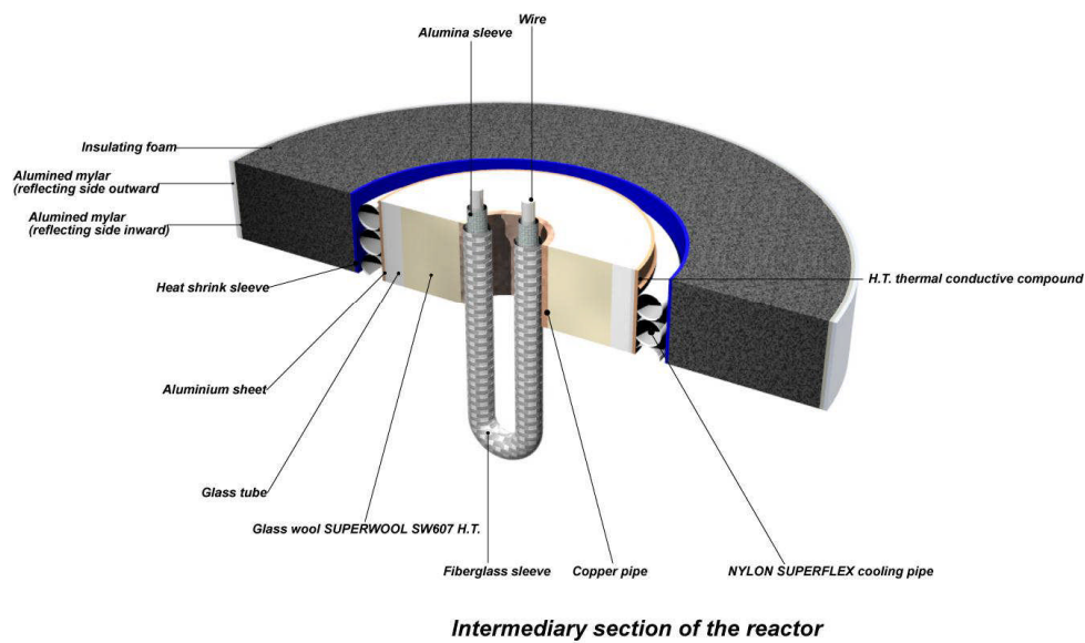
Figure 16. Schematic, fully detailed, of head of the reactor. It is shown only 1 over the 3 wires used.
