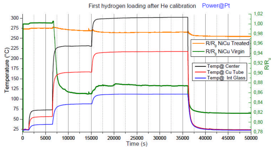
Figure 24. First loading with H 2 at 8Atm.
