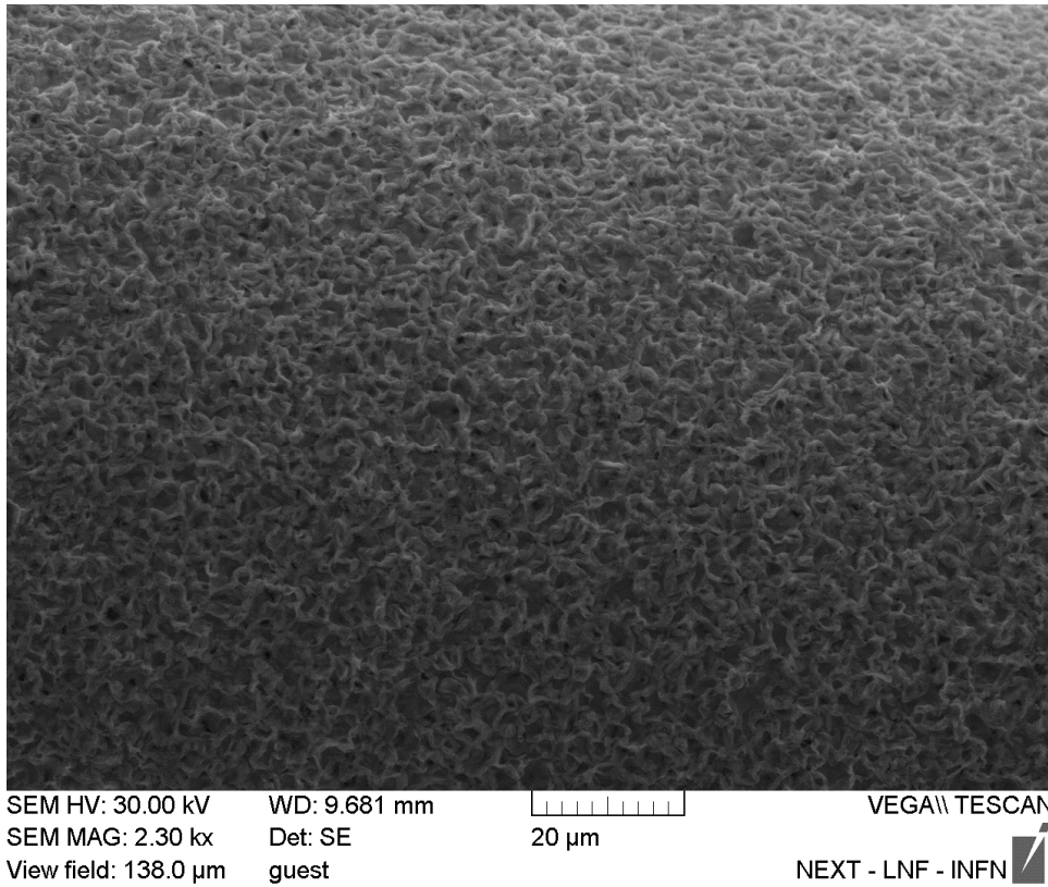
Figure 8. SEM . I=2900mA, 2m. Temperature too-large: re-sintering effect.
