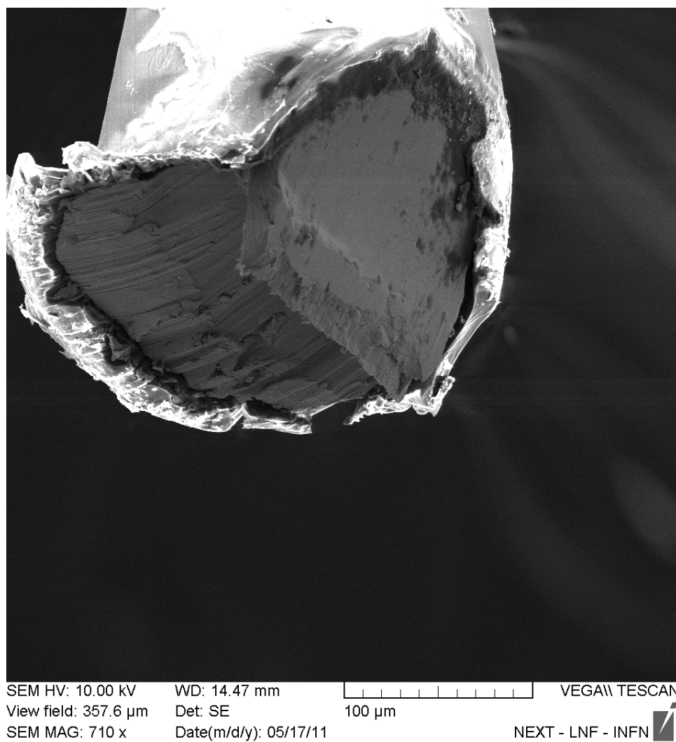
Figure 2. SEM. Cross section of virgin wire, as provided by Isabellenhutte, with "plastic" cover at the surface (lighter area at the microphotography).
