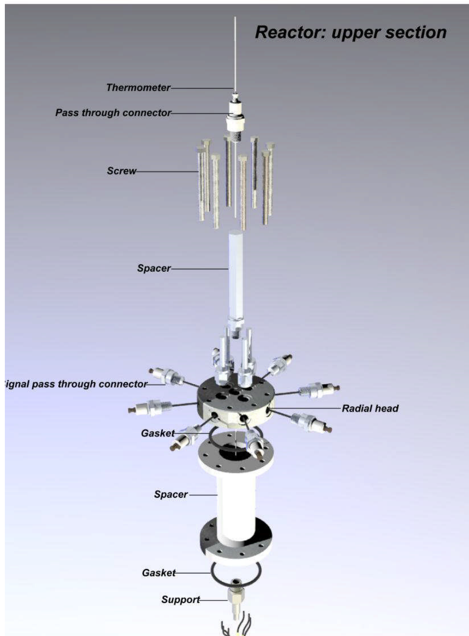
Figure 17. Schematic of head assembly with electric connections
