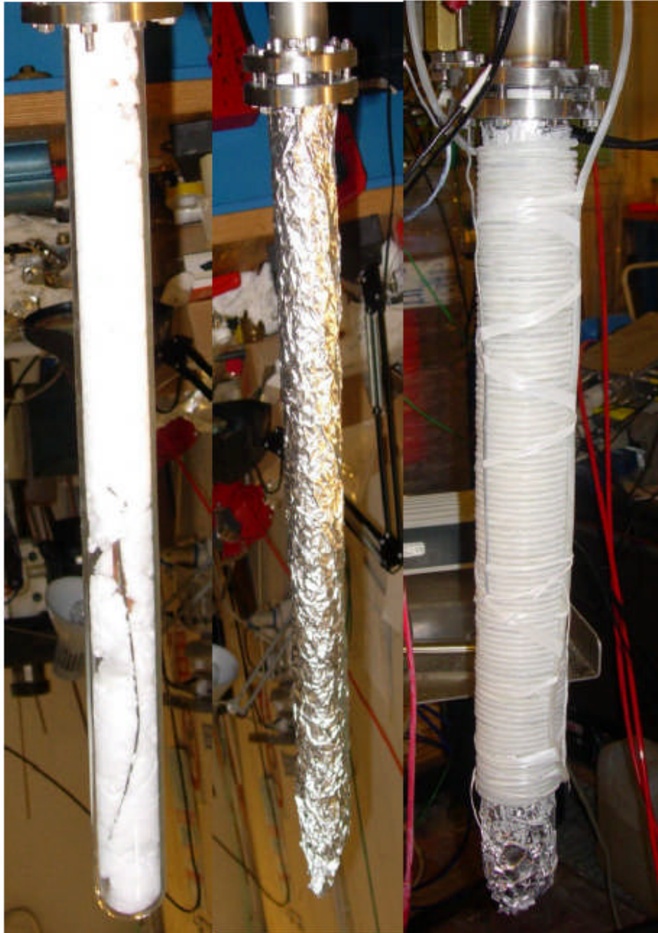
Figure 20. Real reactor: steps 1-3 of assembly.
