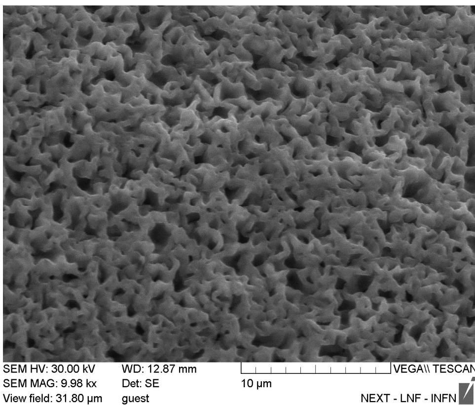
Figure 10. SEM. I=2800mA, 3m. Extra treatments with \text{HNO}_3 at 65%, 500s. Strong reduction of Cu.
