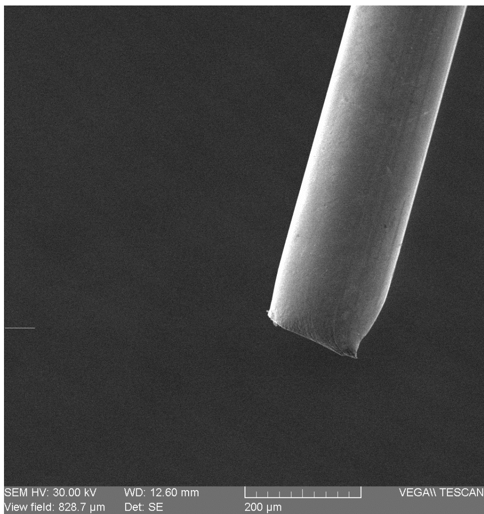
Figure 3. SEM. Wire after removing plastic cover by Joule heating at I=2000\text{mA} , 5m.
