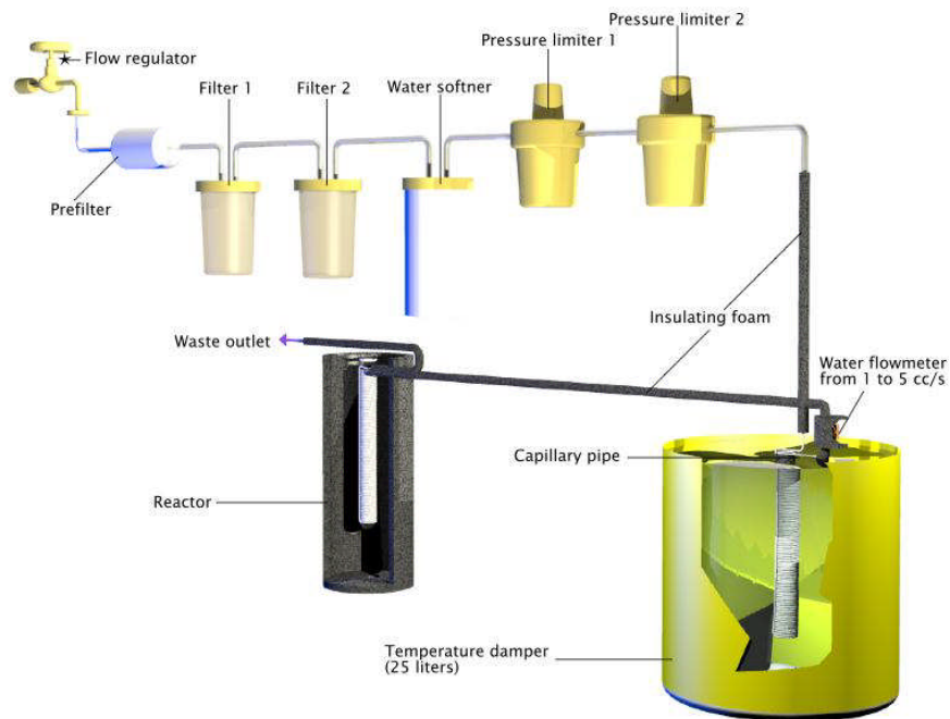
Figure 23. Schematic of the cooling system
