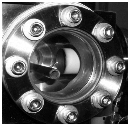
FIGURE 2. View of anode (left) and cathode (right).
