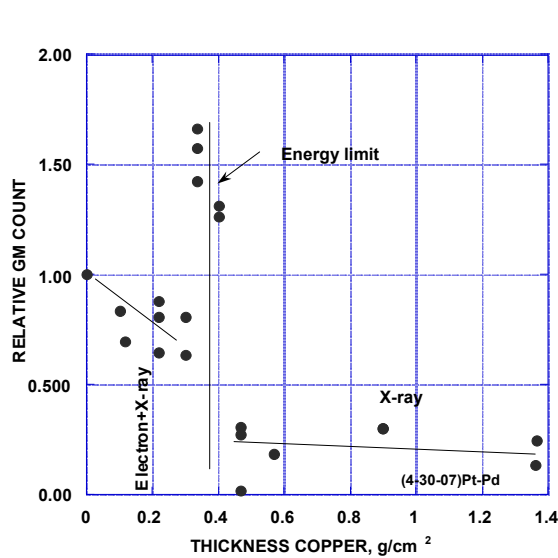
FIGURE 9. Effect of copper absorbers on the amount of radiation reaching the GM tube from a Pd+Pt cathode.
