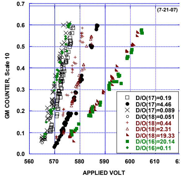
FIGURE 10. Effect of voltage on emission at various D/O atom ratios and with various isotopic compositions of oxygen.
